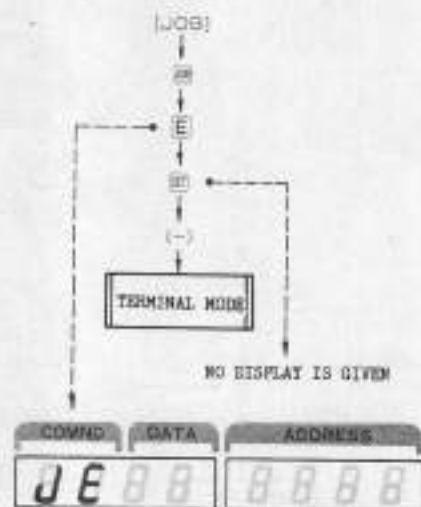
Fig. 3-12 Flowchart of TERMINAL Command
