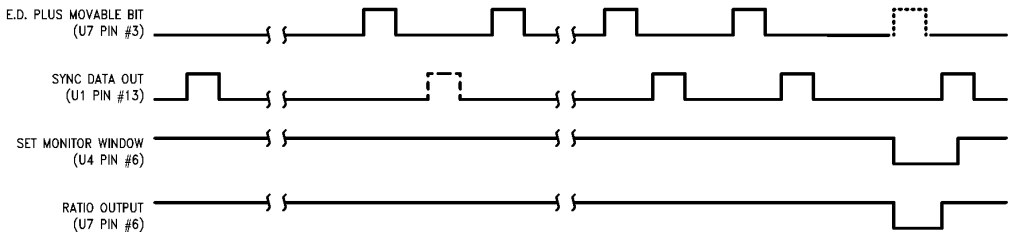
FIGURE 8. Essential Waveform Diagrammatic Representation of the DP8462 Evaluation Board
