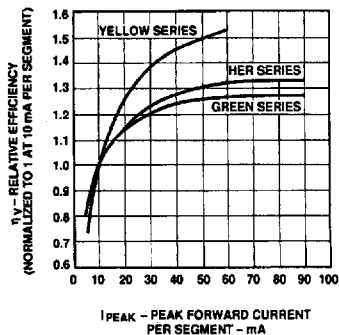
Figure 13. Relative Luminous Efficiency (Luminous Intensity per Unit Current) vs. Peak Current.
