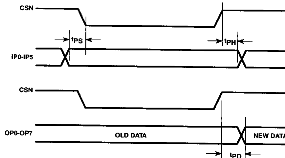
Figure 5. Port Timing
