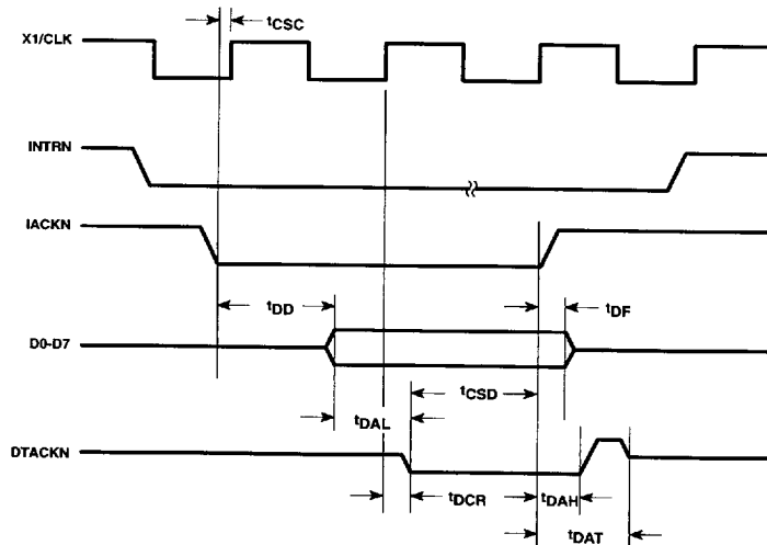
Figure 4. Interrupt Cycle Timing
