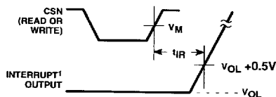
Figure 5. Port Timing
