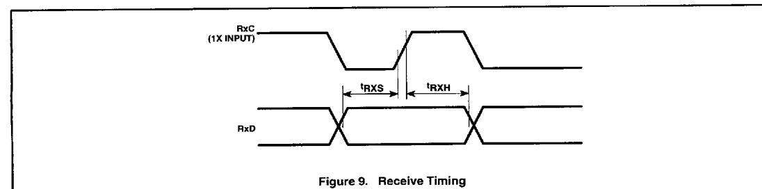
Figure 9. Receive Timing
