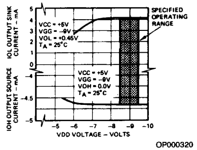
Output Current Versus VDD Supply Voltage
