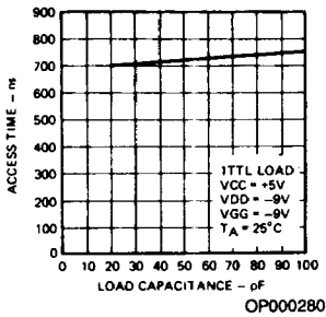
Access Time Versus Load Capacitance
