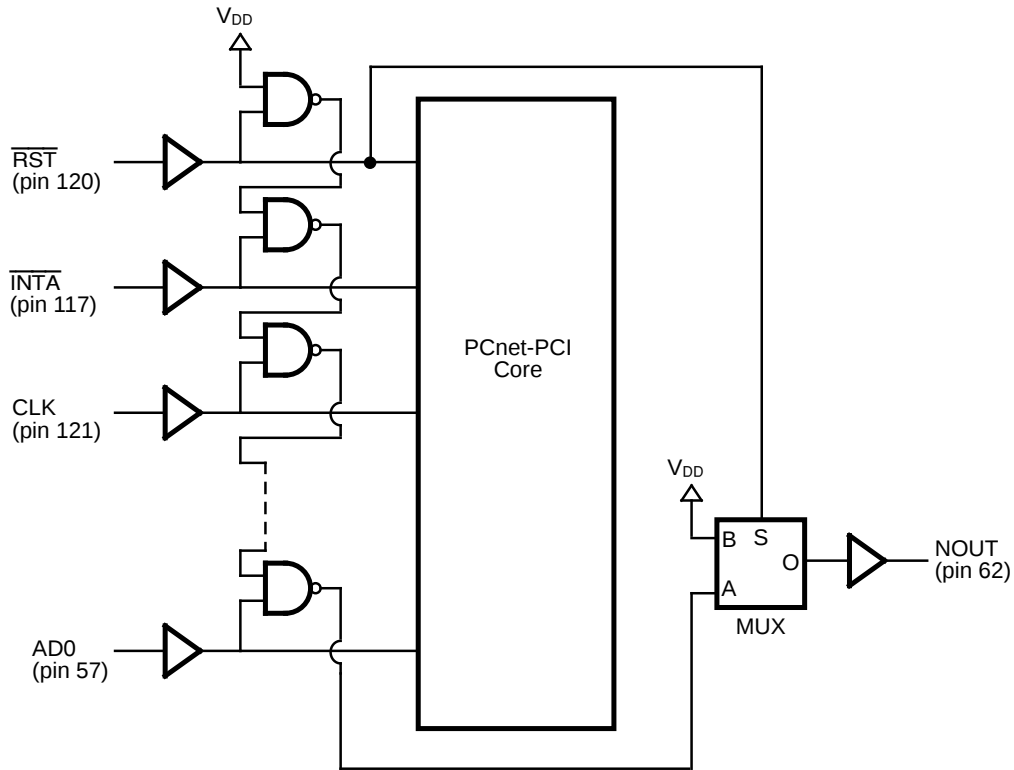
Figure 30. NAND Tree
