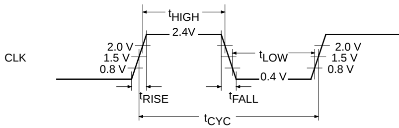
CLK Waveform
