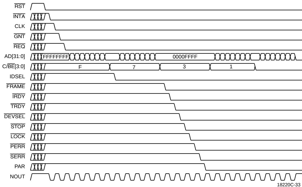
Figure 31. NAND Tree Waveform
