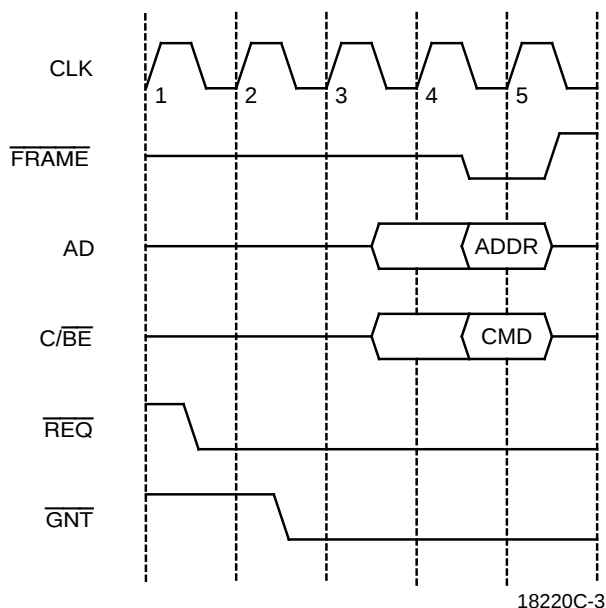
Figure 1. Bus Acquisition
