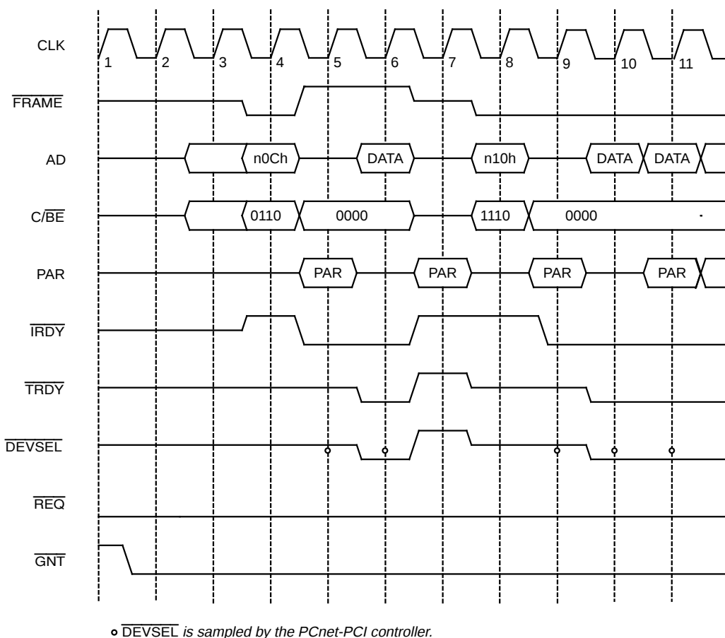
Figure 16. Burst Alignment
