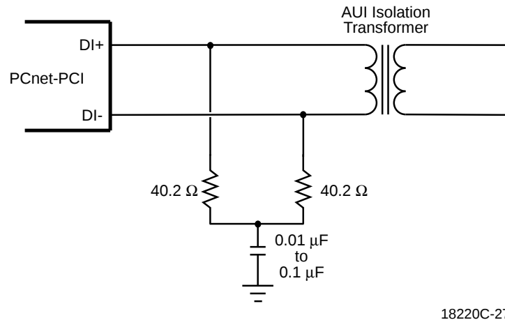
Figure 25. Differential Input Termination
