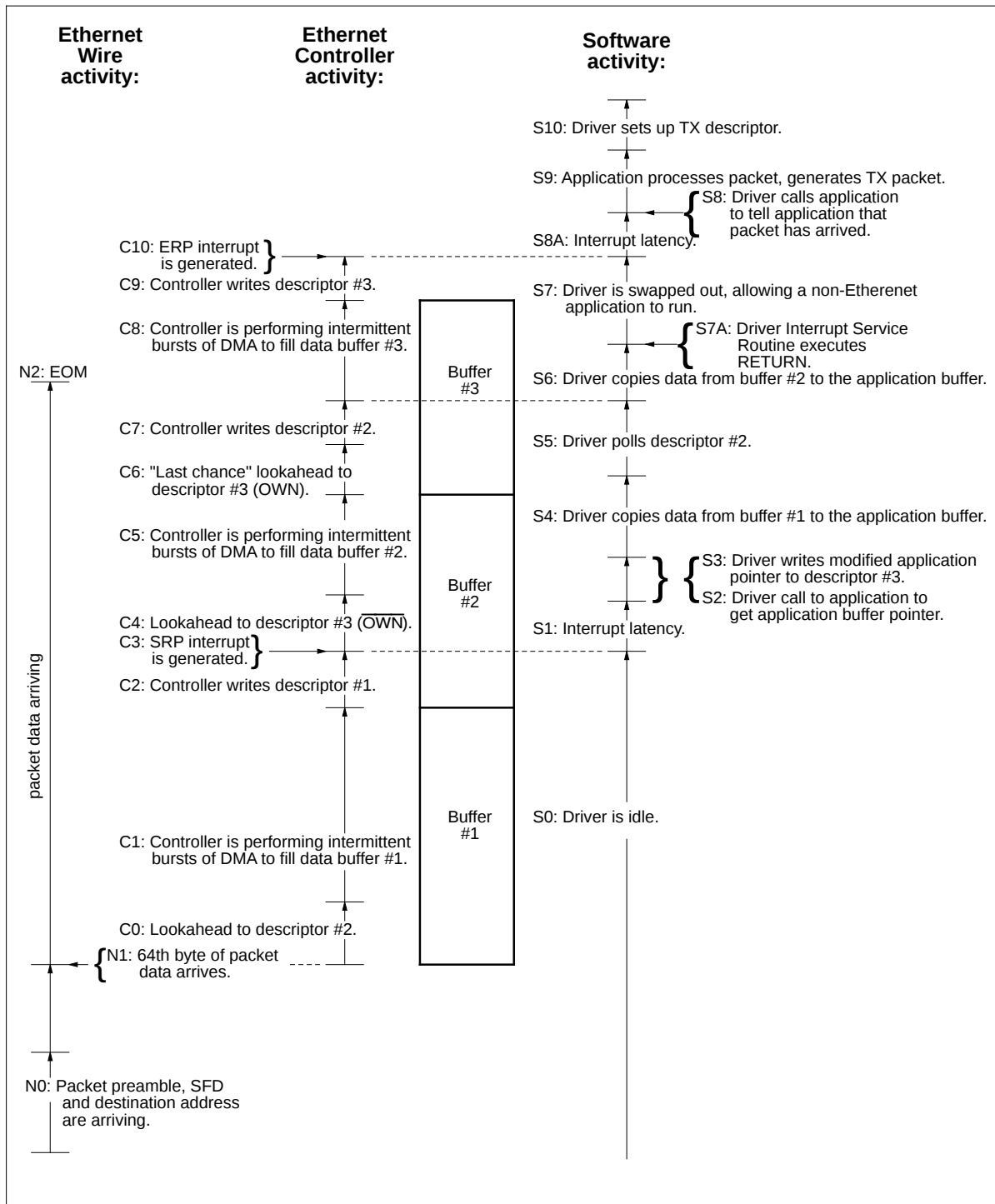
Figure D3. LAPP Timeline for TWO-INTERRUPT Method
