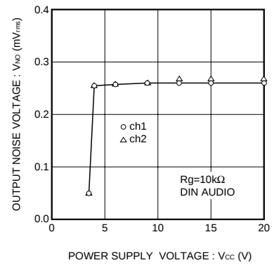
Fig.6 Output noise voltage vs. Power supply voltage
