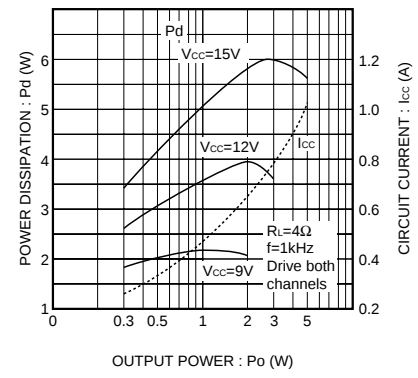
Fig.12 Power dissipation vs. Power supply voltage ( R_L=4\Omega )
