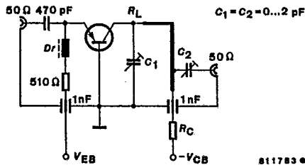
Test circuit for: G_{pb}
