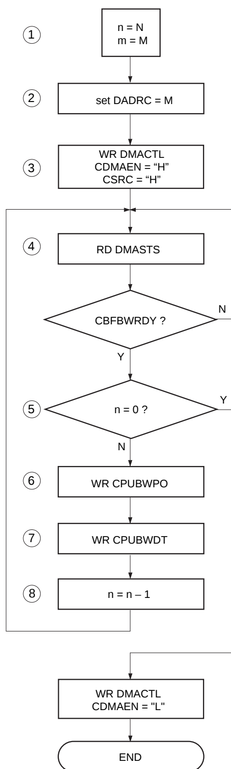
Fig. 6.1 CPU buffer write control
