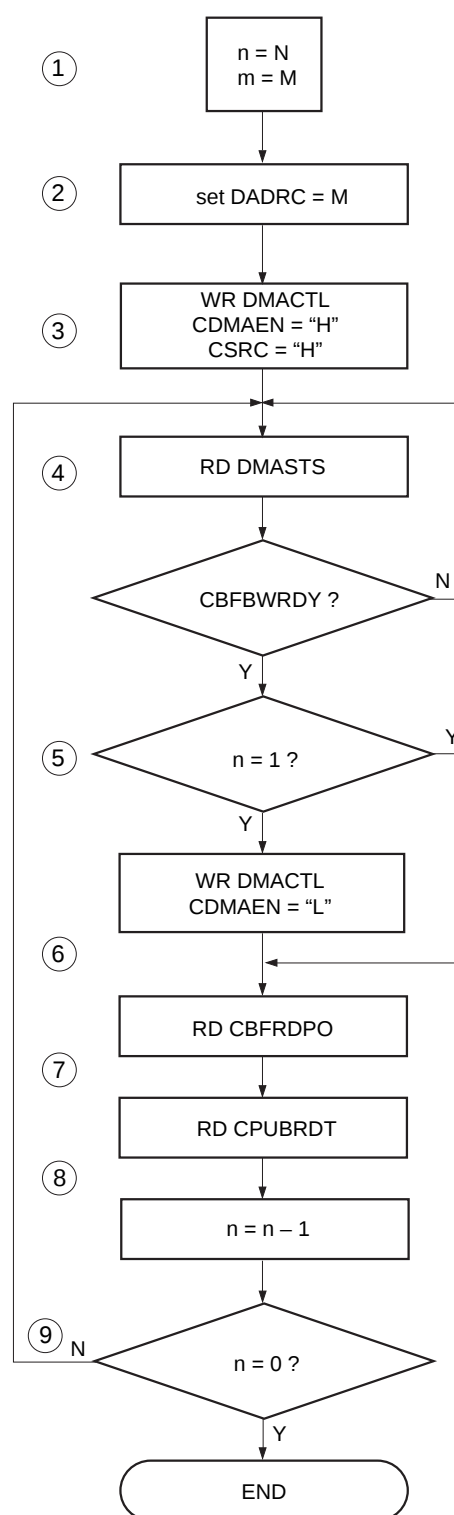
Fig. 6.2 CPU buffer read control
