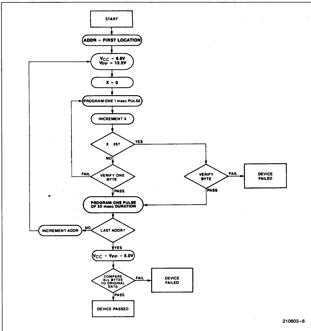
Figure 3. M27128A Intelligent Programming™ Flowchart
