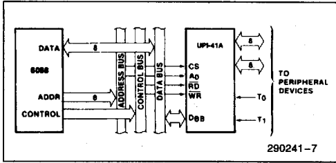
Figure 1. 8085A-8741A Interface
