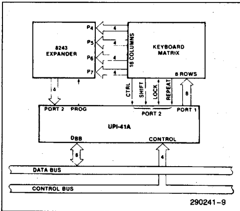
Figure 3. 8741A-8243 Keyboard Scanner
