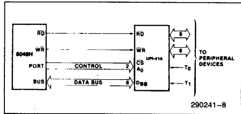
Figure 2. 8048H-8741A Interface
