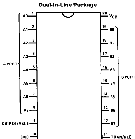
Top View Order Number DP8303AN See NS Package Number N20A
