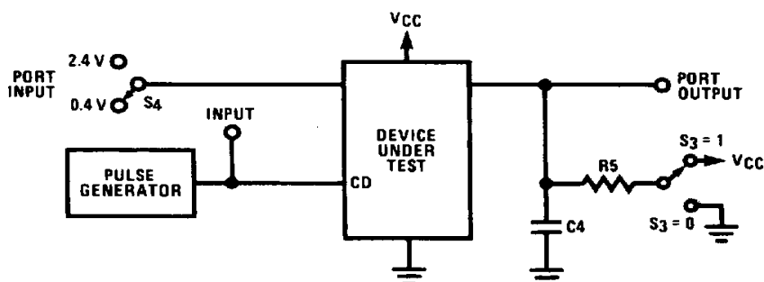
FIGURE C. Propagation Delay to/from TRI-STATE from CD to A Port or B Port
