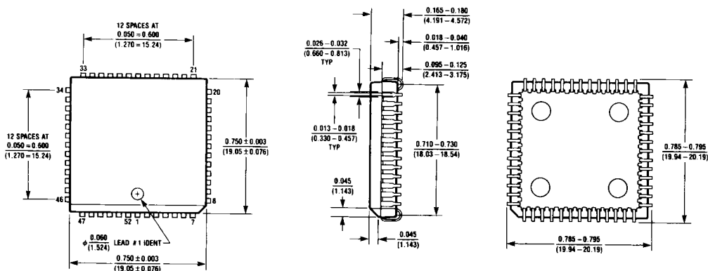
Plastic Leaded Chip Carrier (V) Order Number DP8473V NS Package Number V52A
