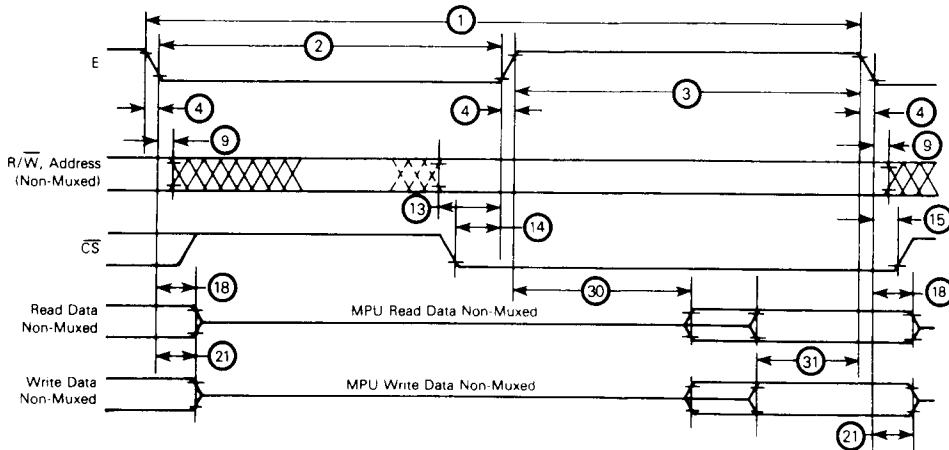
FIGURE 1 - BUS TIMING
