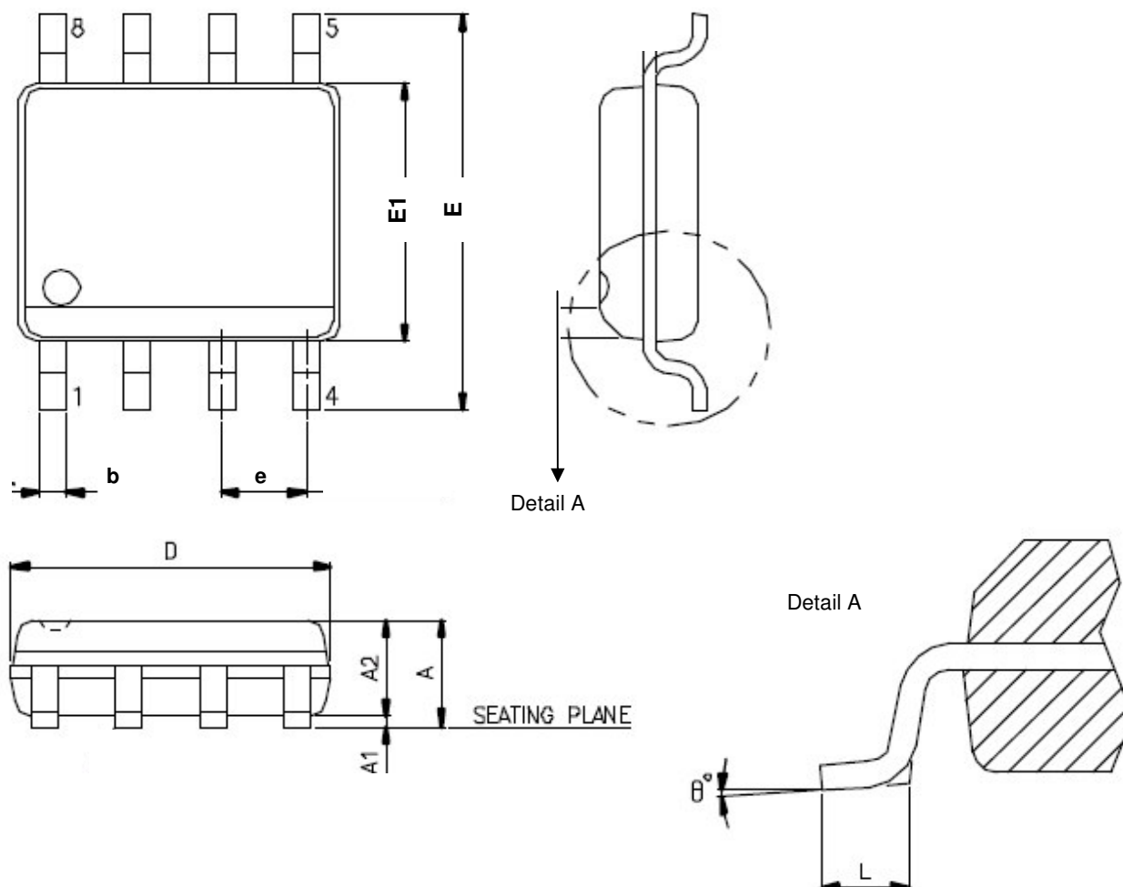
Figure 26. SOP 8 ( 150 mil )
