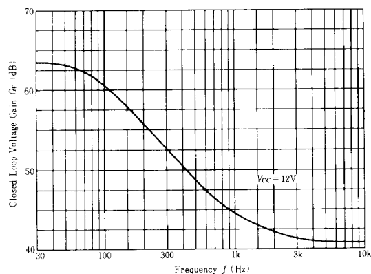
CLOSED LOOP VOLTAGE GAIN OF PREAMP. PLUS LINE AMP. VS. FREQUENCY
