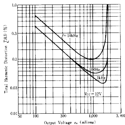
TOTAL HARMONIC DISTORTION OF PREAMP. PLUS LINE AMP. VS. OUTPUT VOLTAGE
