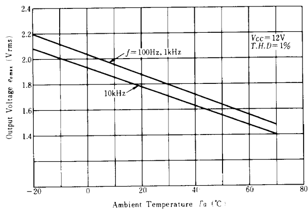
OUTPUT VOLTAGE OF LINE AMP.(REC) VS. AMBIENT TEMPERATURE
