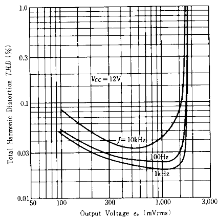
TOTAL HARMONIC DISTORTION OF LINE AMP(REC) VS. OUTPUT VOLTAGE
