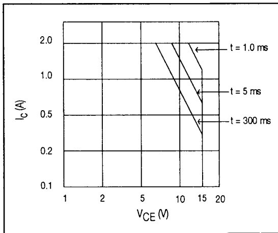
Figure 3 ASO of Output Stages
