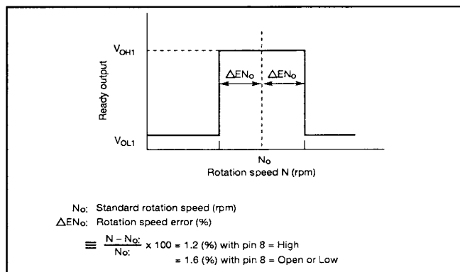
Figure 4 Operation of Ready Circuit
