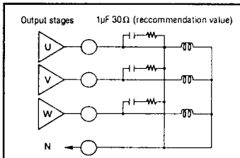
Figure 1 Snubber circuit
