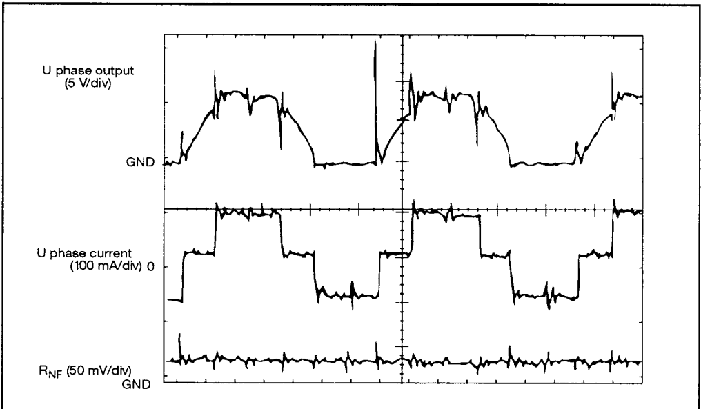
Figure 6 Waveform on Actual Application (3.5" 8 poles motor)
