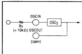
Figure 2 Application for external CLK
