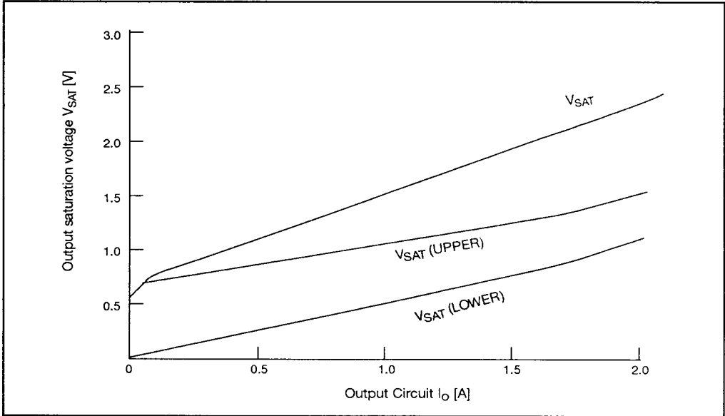
Figure 5 V_{sat} vs I_o
