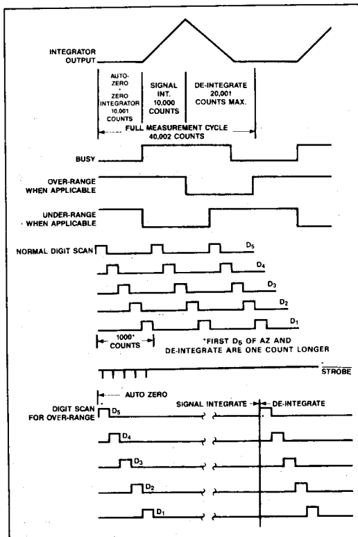
Figure 4. Timing Diagram
