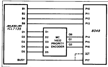
Figure 13. μP Interface
