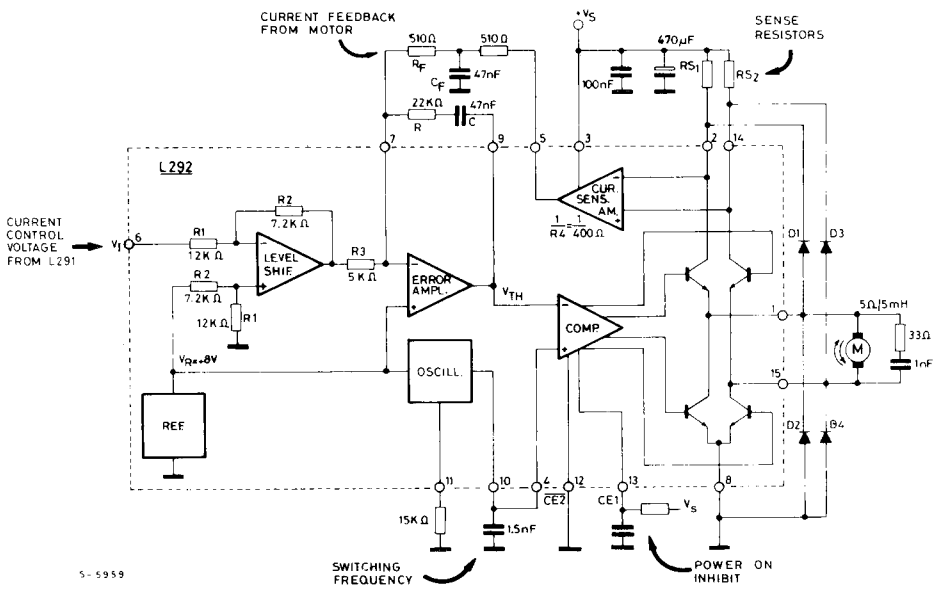
Fig. 7 - The L292 switchmode driver receives a control voltage from the L291 and delivers a switchmode regulated current to the motor.
