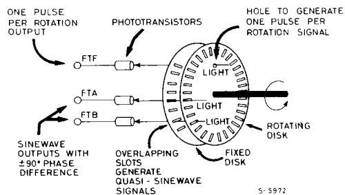
Fig. 3 - The system operates with an optical encoder of the type shown schematically here. It generates two signals 90^\circ out of phase plus a one pulse-per-rotation signal.
