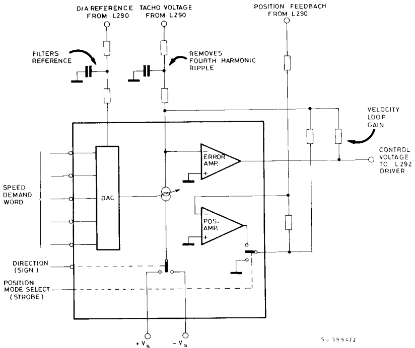
Fig. 6 - The L291 links the system to the microprocessor. It contains the system DA converter, main error amplifier and position amplifier.
