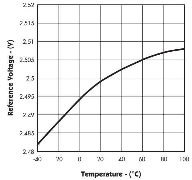
FIGURE 11. — TEMPERATURE DRIFT
