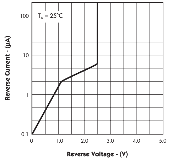
FIGURE 9. — REVERSE CHARACTERISTICS
