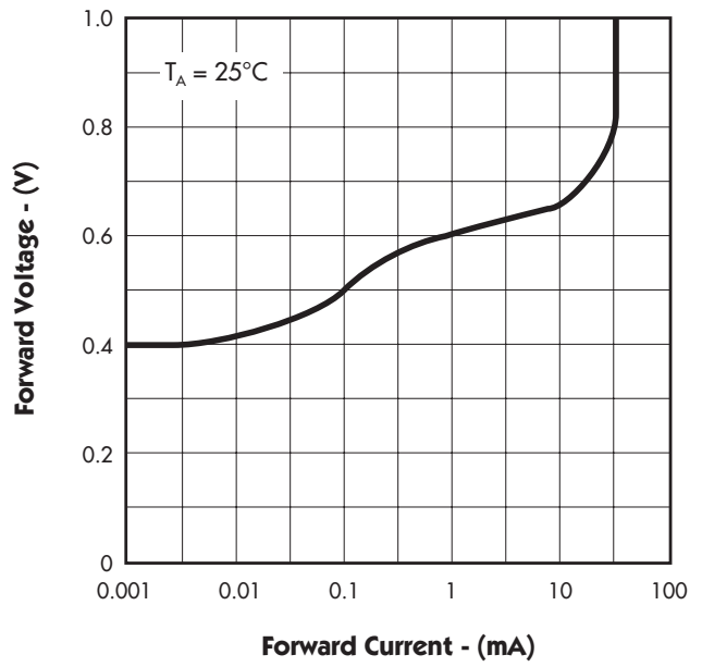
FIGURE 10. — FORWARD CHARACTERISTICS
