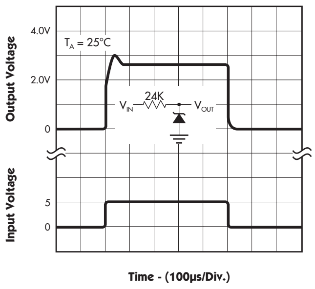
FIGURE 8. — RESPONSE TIME
