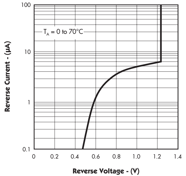
FIGURE 2. — REVERSE CHARACTERISTICS
