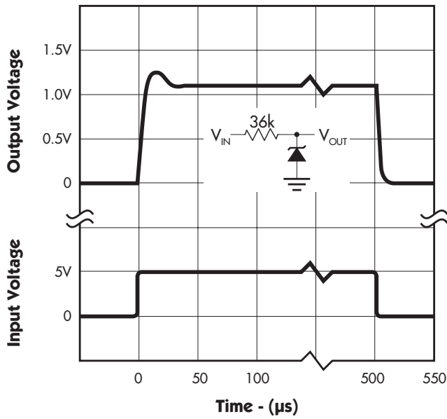
FIGURE 1. — RESPONSE TIME
