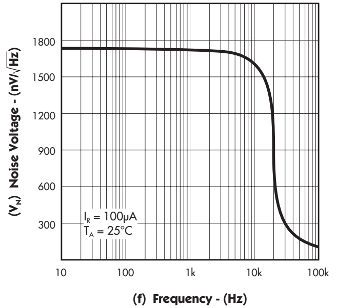
FIGURE 13. — NOISE VOLTAGE
