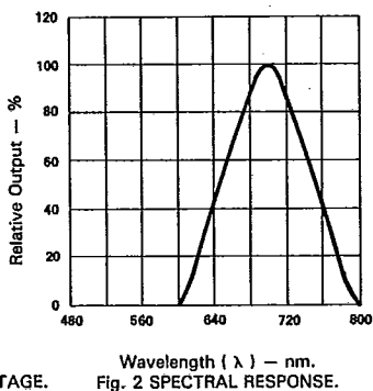
Fig. 2 SPECTRAL RESPONSE.
