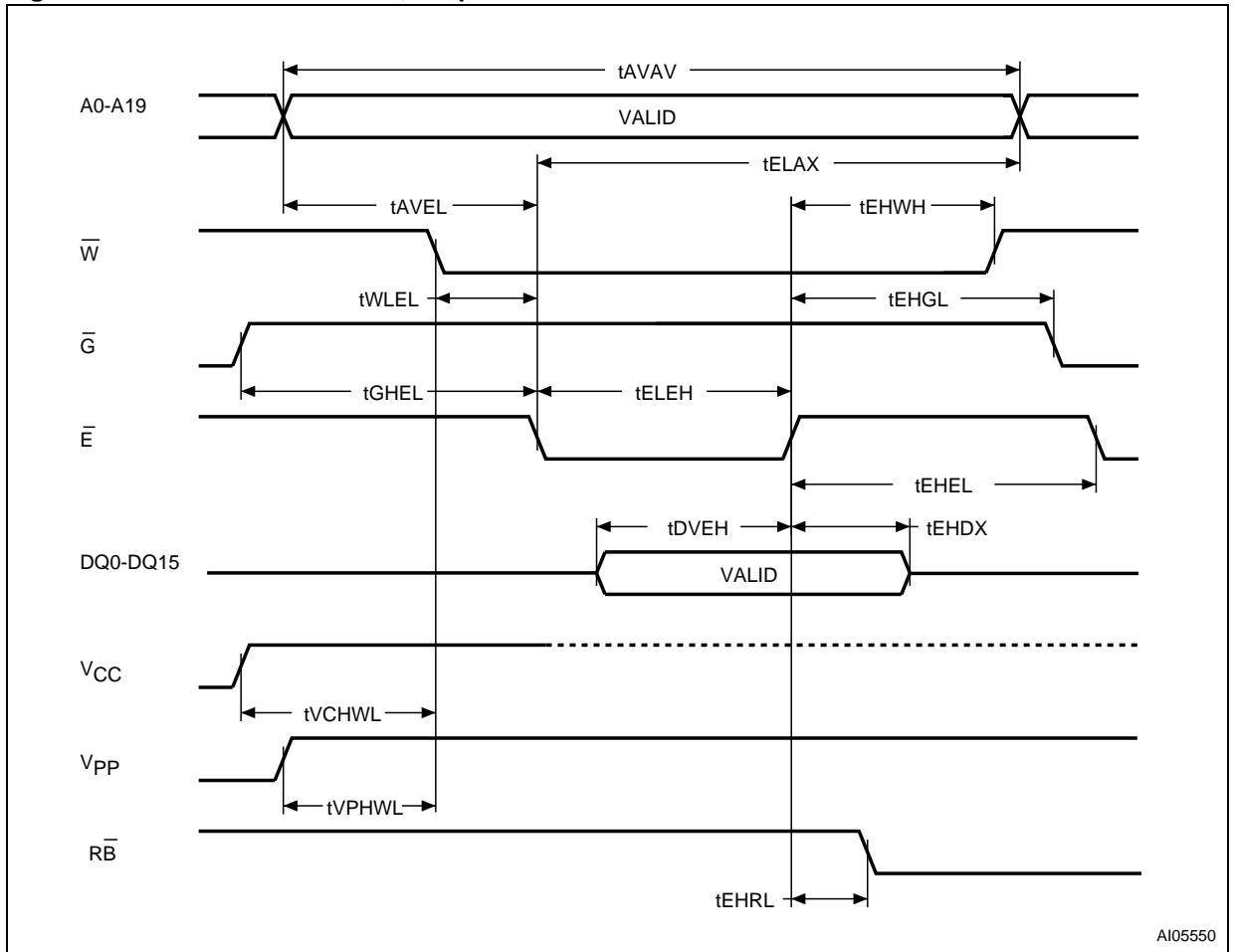
Figure 13. Write AC Waveforms, Chip Enable Controlled
