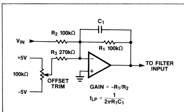
Figure 18. Circuit for DC Offset Adjustment
