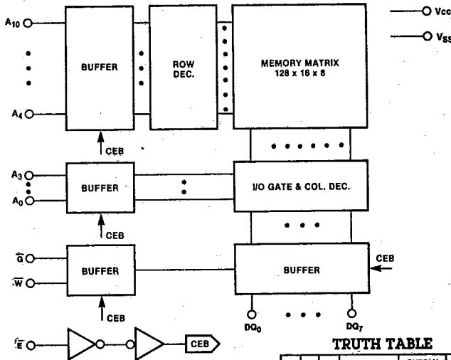
MB8416 BLOCK DIAGRAM
