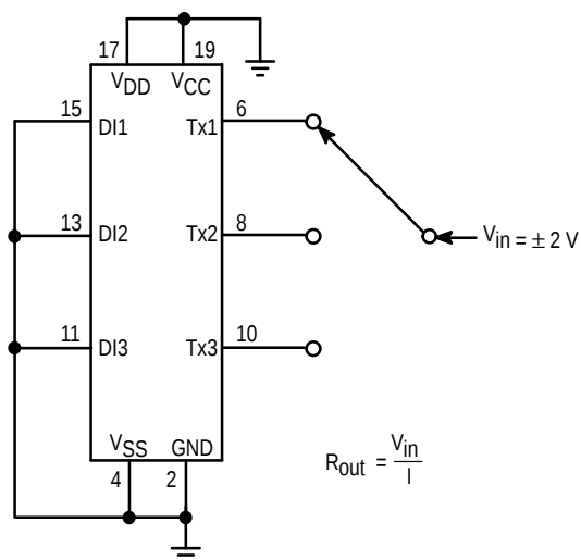
Figure 1. Power-Off Source Resistance
