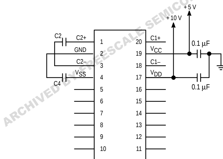
Figure 6. Two Supply Configuration (MC145407 Generates VSS Only)
