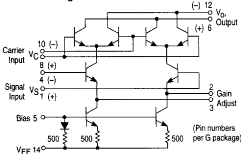
Figure 23. Circuit Schematic
