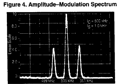
Figure 4. Amplitude-Modulation Spectrum
