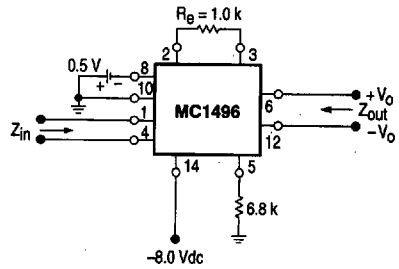
Figure 6. Input-Output Impedance
