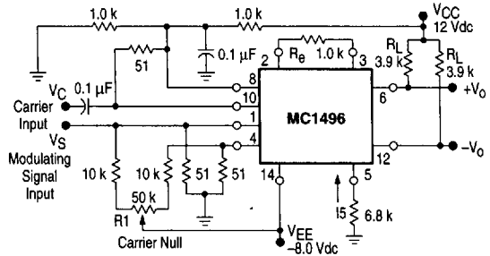
Figure 27. Balanced Modulator-Demodulator
