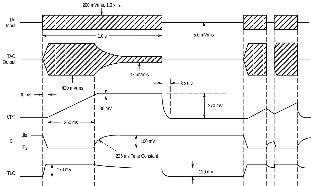
Figure 17. Idle \longleftrightarrow Transmit Timing
