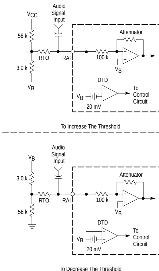
Figure 33. Adjusting Dial Tone Detector Threshold (AC Coupled)
