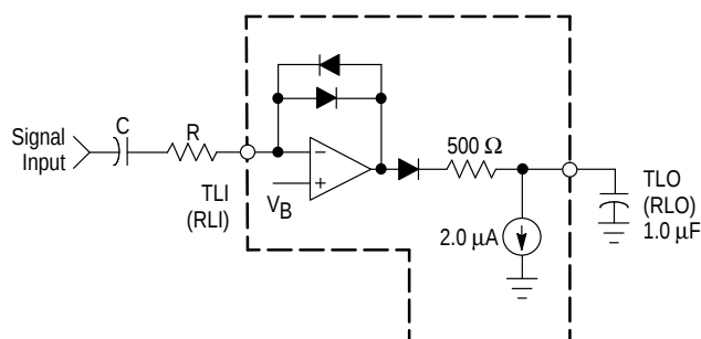
Figure 26. Level Detector
