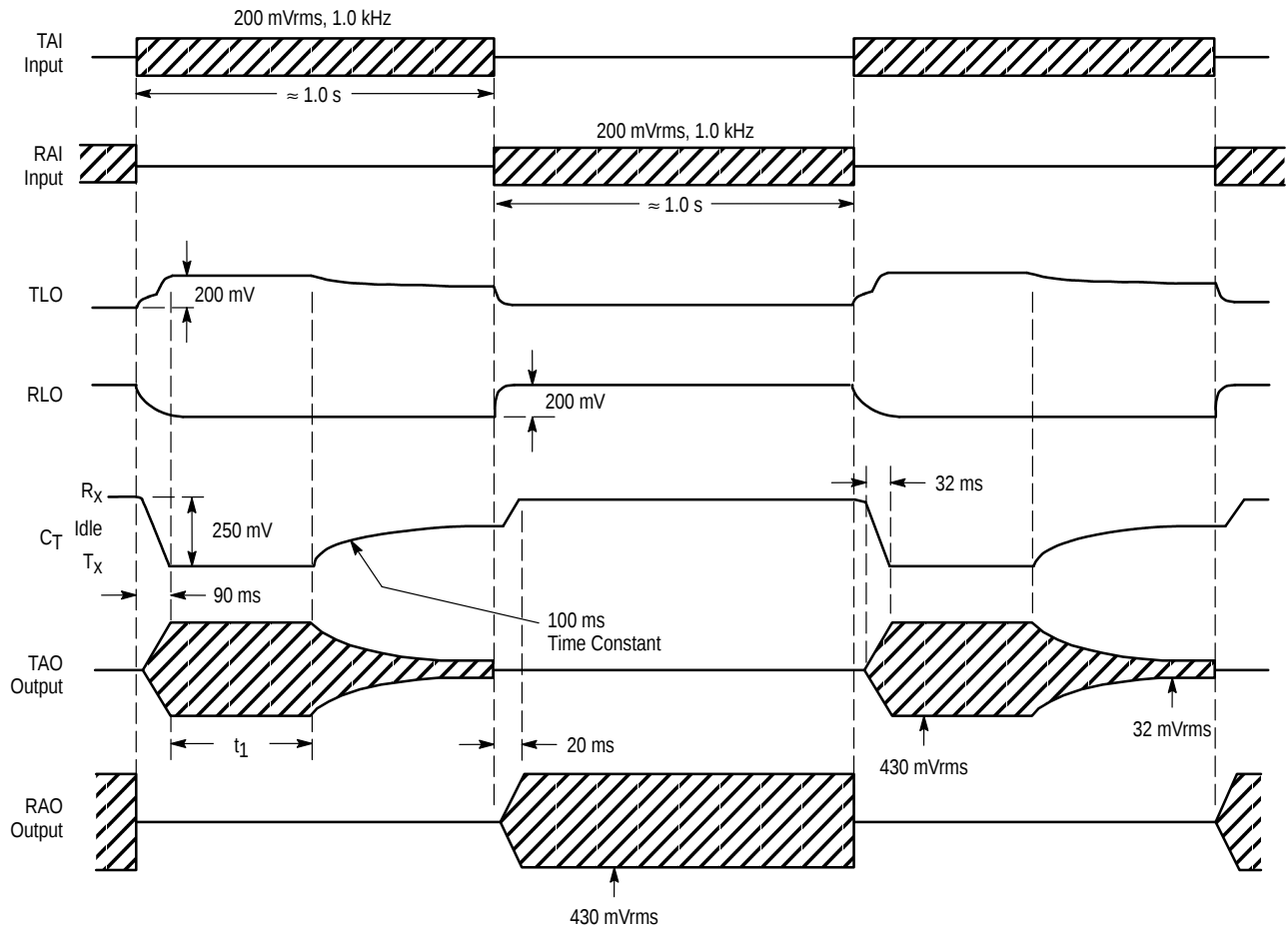
Figure 21. Transmit \longleftrightarrow Receive Timing (Long Cycle Timing)
