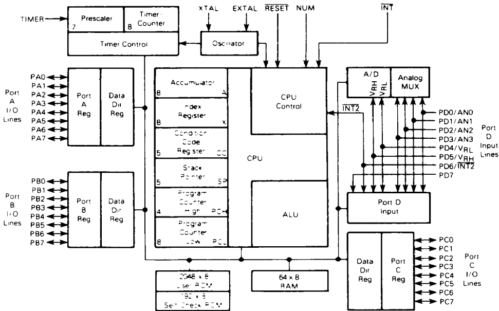
BLOCK DIAGRAM
