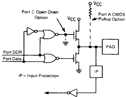
Figure 16. Ports A and C Logic Diagram
