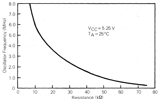
FIGURE 12 — TYPICAL FREQUENCY SELECTION FOR RESISTOR OSCILLATOR OPTION
