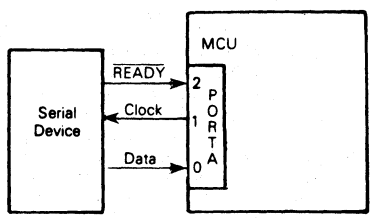
FIGURE 19 — BIT MANIPULATION EXAMPLE
