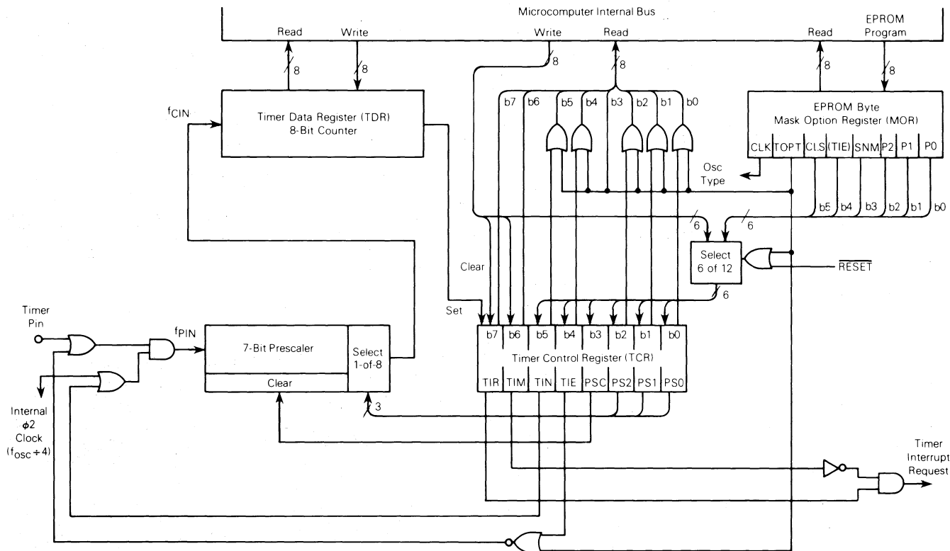
FIGURE 7 — MC68705P5 TIMER FUNCTIONAL BLOCK DIAGRAM
