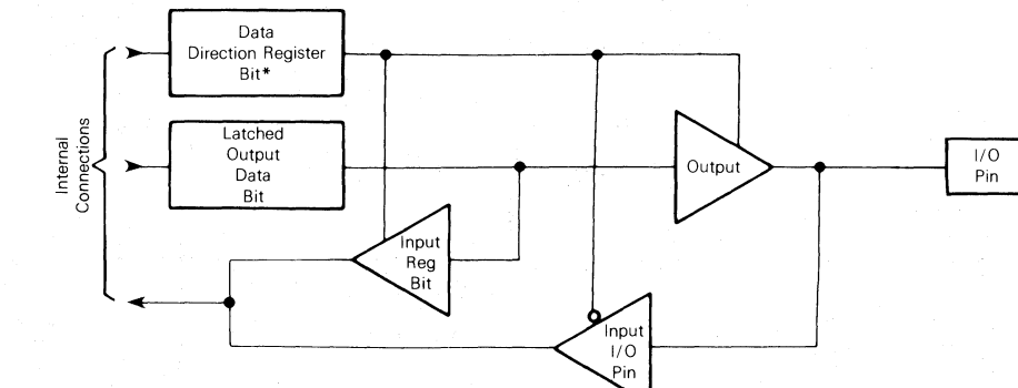
FIGURE 15 – TYPICAL PORT I/O CIRCUITRY
