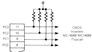
Port C, Bits 0-3 Programmed as Output, Driving CMOS Loads, Using External Pullup Resistors
