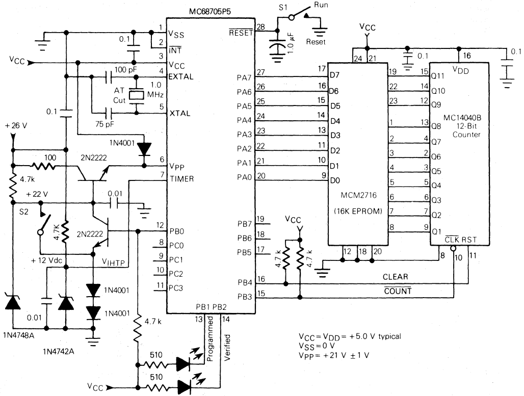
FIGURE 18 — PROGRAMMING CONNECTIONS SCHEMATIC DIAGRAM
