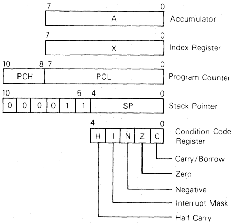
FIGURE 6 — PROGRAMMING MODEL
