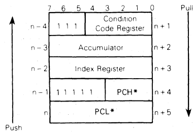
FIGURE 5 — INTERRUPT STACKING ORDER
