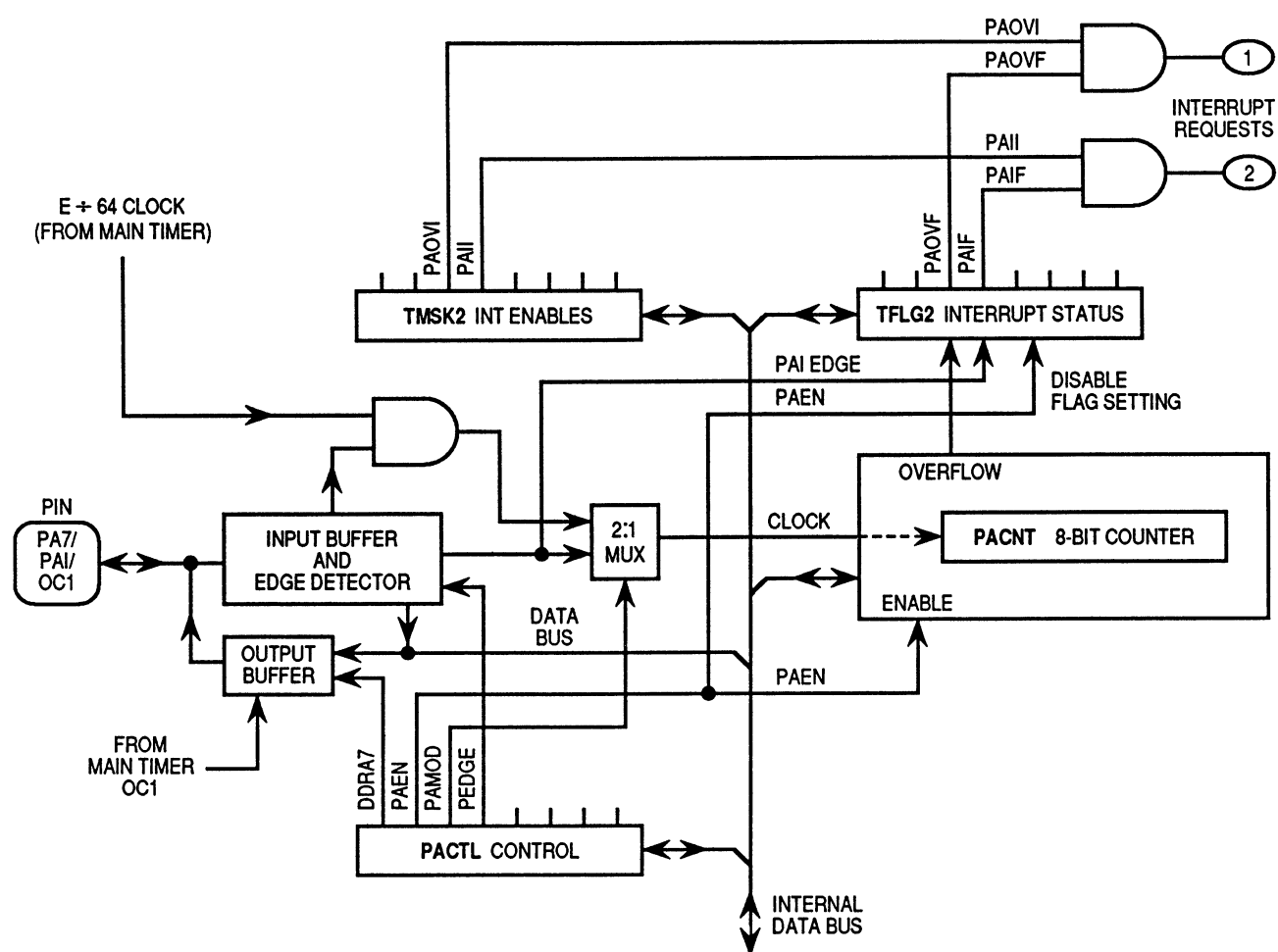
Figure 9–3. Pulse Accumulator
