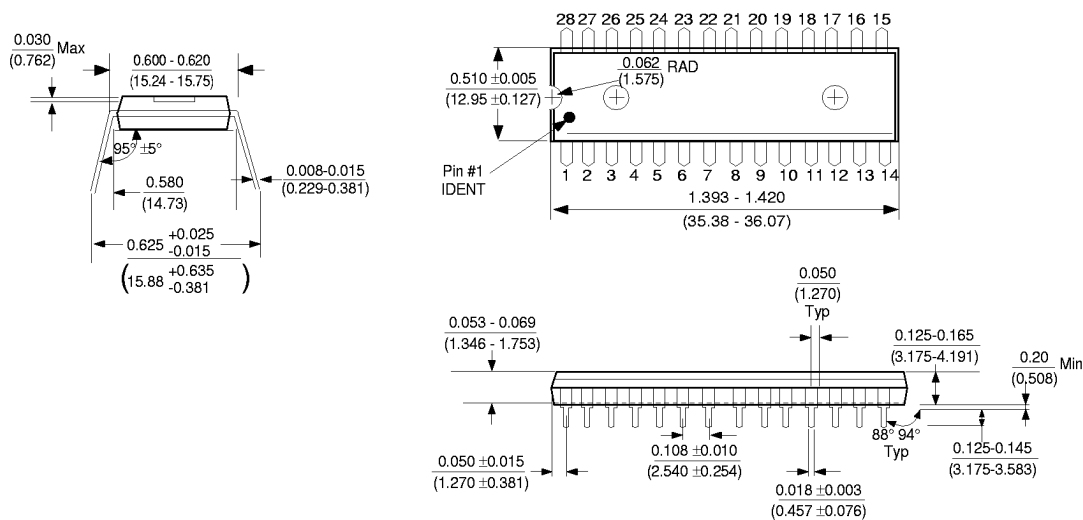
28-Lead Plastic One-Time-Programmable Dual-In-Line Order Number NM27C512N Package Number N28B
