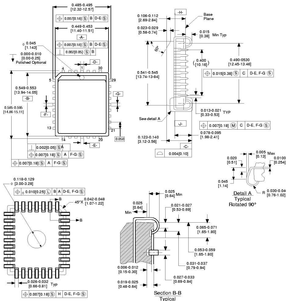
32-Lead Plastic Leaded Chip Carrier (PLCC) Order Number NM27C512V Package Number VA32A
