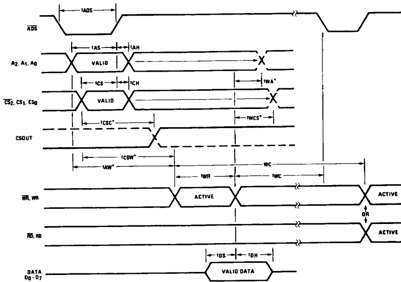
Write Cycle
