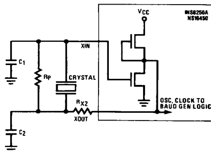
Typical Oscillator Networks
