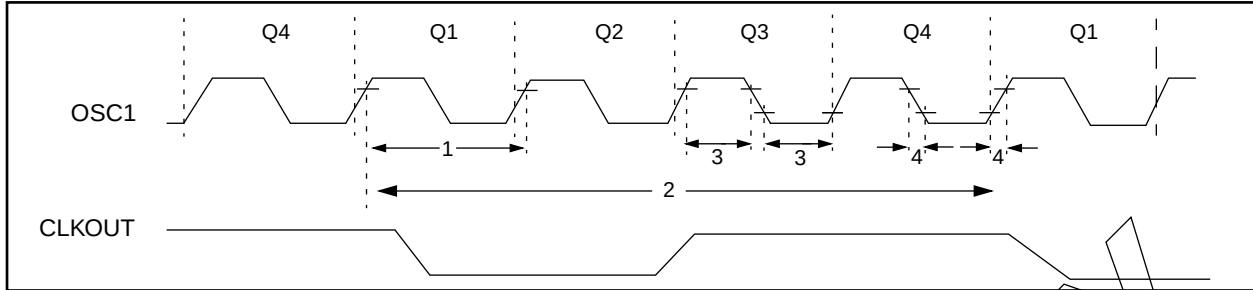
FIGURE 12-2: EXTERNAL CLOCK TIMING
