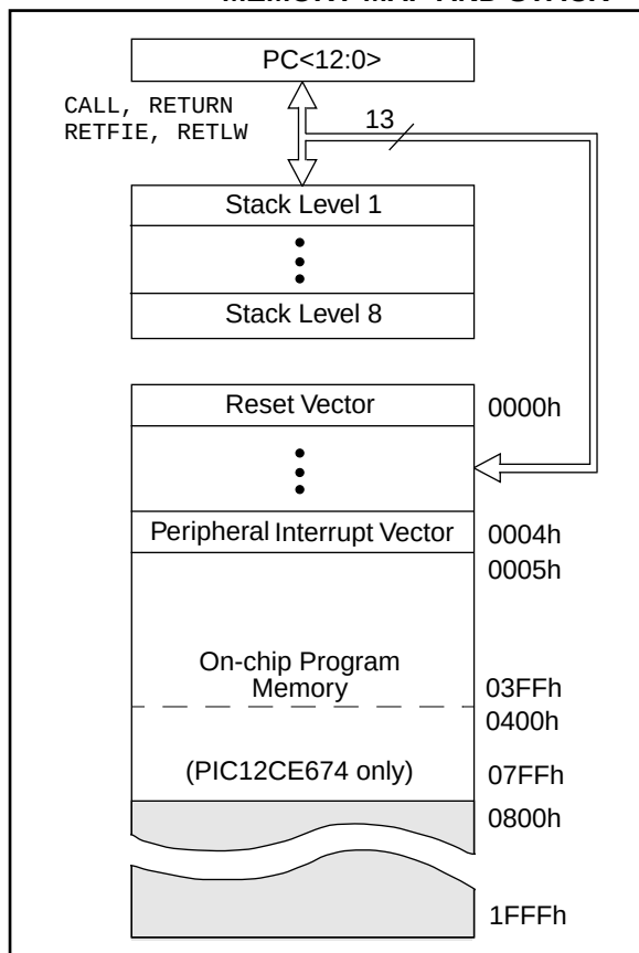
FIGURE 4-1: PIC12CE67X PROGRAM MEMORY MAP AND STACK
