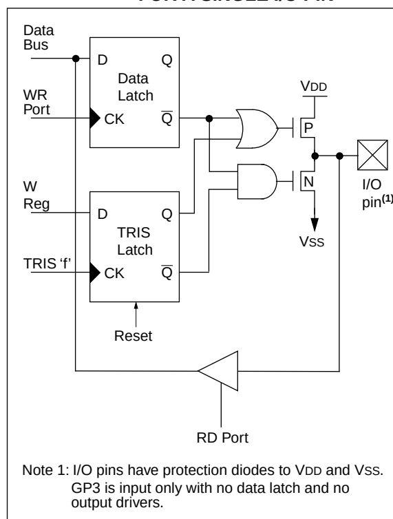
FIGURE 5-1: EQUIVALENT CIRCUIT FOR A SINGLE I/O PIN
