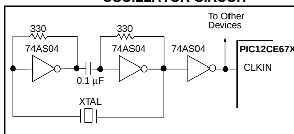
FIGURE 9-5: EXTERNAL SERIES RESONANT CRYSTAL OSCILLATOR CIRCUIT
