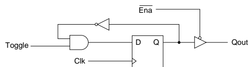
Figure 3-3 Dot Extensions and Architecture-Independence: Circuit 1
