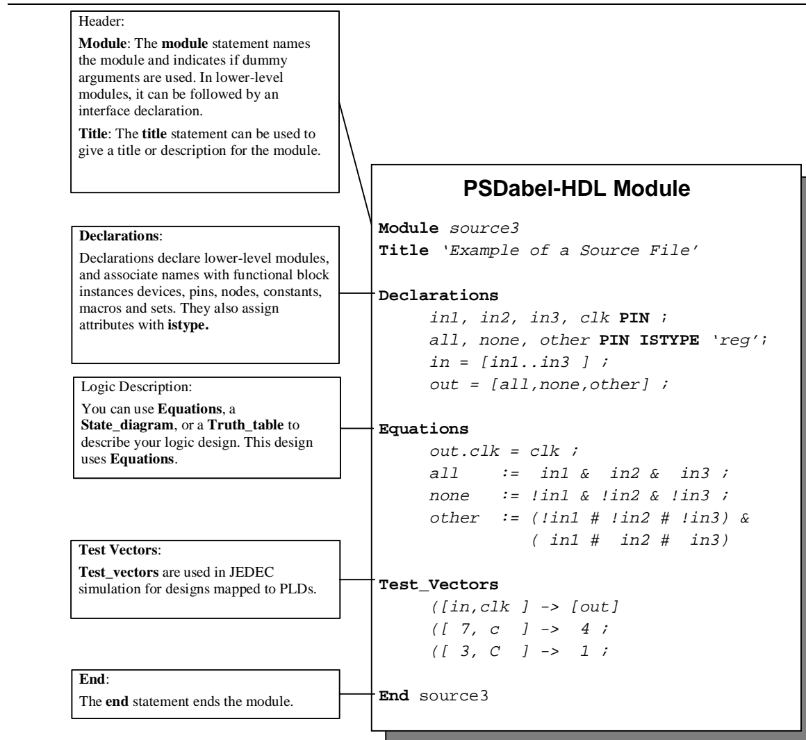
Figure 2-1 PSDabel-HDL Module Structure
