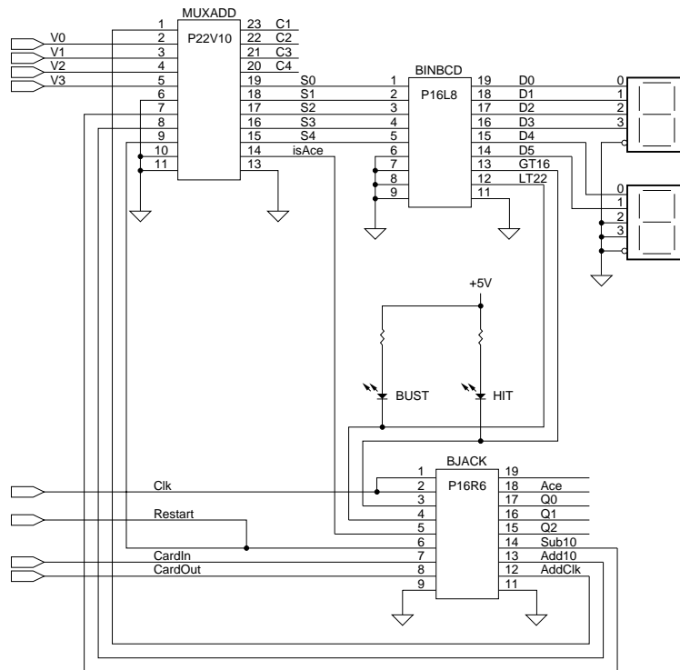
Figure 4-20 Schematic of a Blackjack Machine Implemented in Three PLDs
