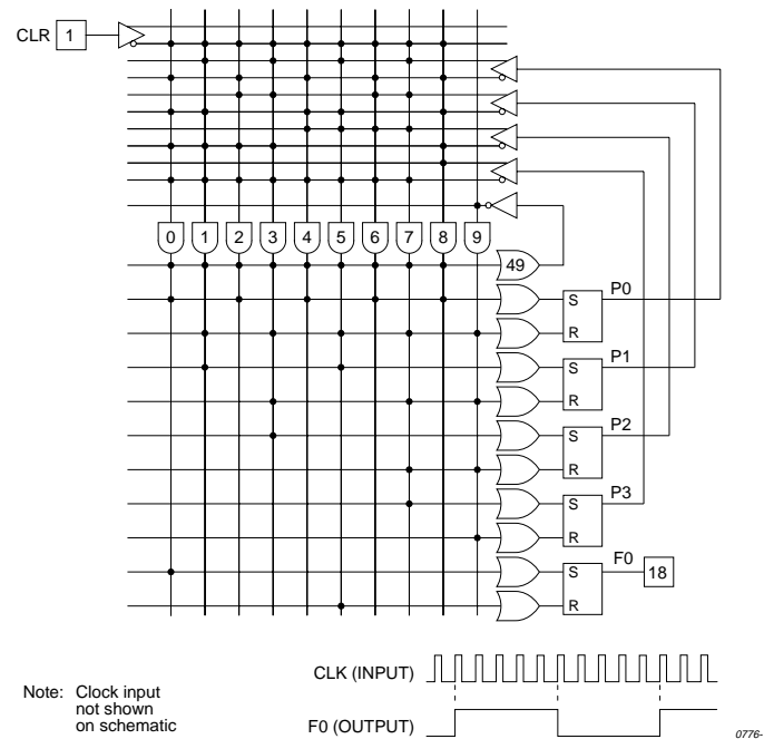
Figure 3-19 Abbreviated F105 Schematic
