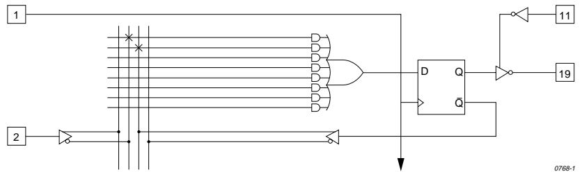
Figure 3-5 Dot Extensions and Architecture-Independence: Circuit 2
