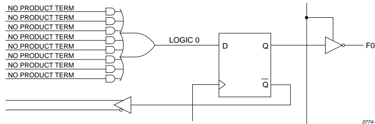
Figure 3-14 D-type Register with False Inputs
