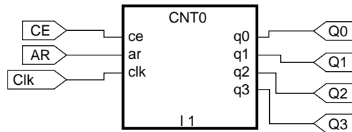
Figure 5-10 Wiring of CNT0
