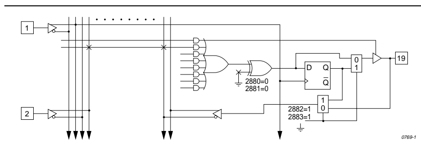
Figure 3-6 Dot Extensions and Architecture-Independence: Circuit 3
