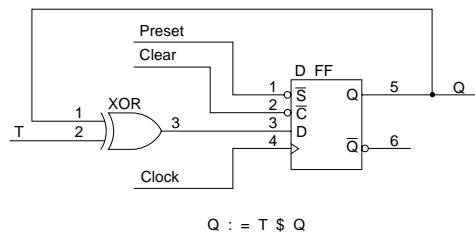
Figure 3-11 T Flip-flop Emulation Using D Flip-flop
