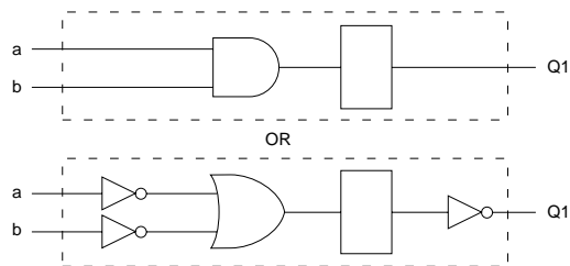
Figure 3-2 Pin-to-pin Macrocell
