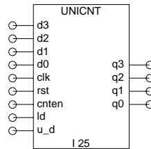
Figure 4-7 Block Diagram: 4-bit Universal Counter
