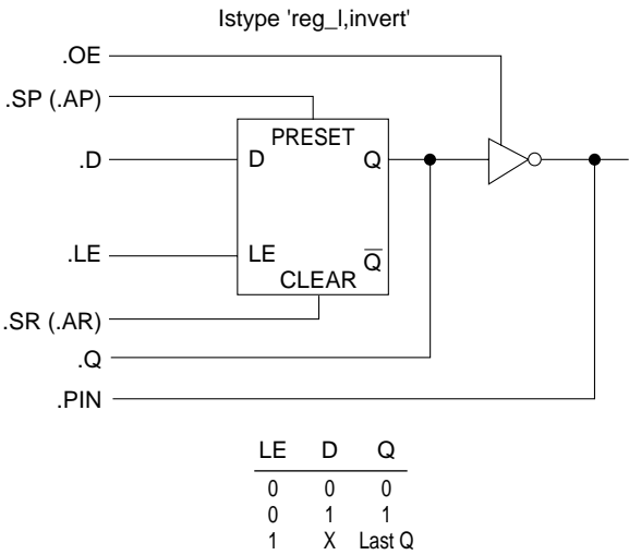
Figure 5-2 Pin-to-pin Dot Extensions in a Non-inverted Output Architecture
