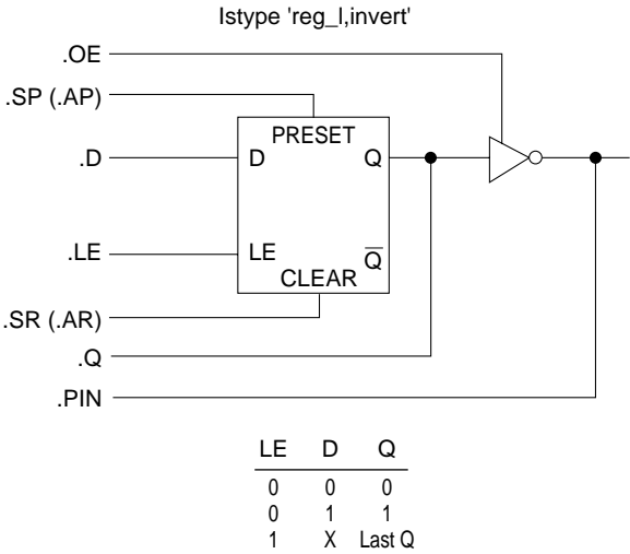
Figure 5-8 Detailed Dot Extensions for a Latch with Active Low Latch Enable
