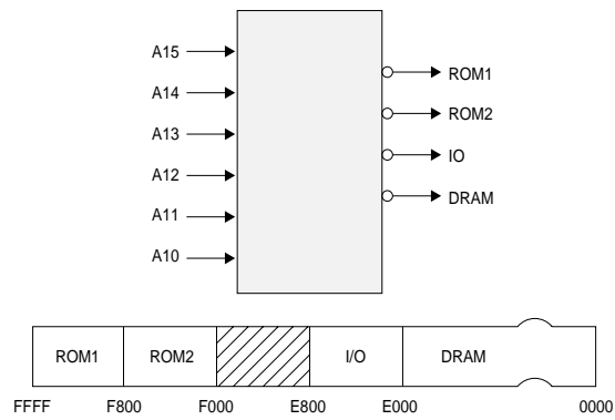
Figure 4-1 Block Diagram: Memory Address Decoder
