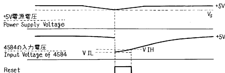
〔Fig. 4〕Example of operation with minimum RESET pulse width.
