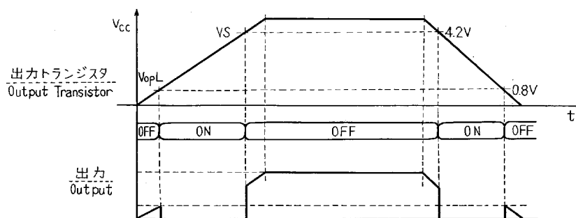
[Fig. 1] PST519 の動作/Operation of PST519
