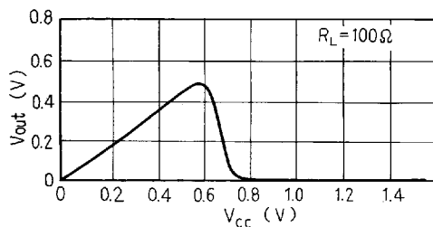
■動作限界電圧/Threshold Operating Voltage
