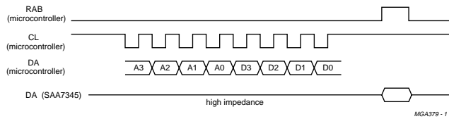
Fig.5 Microcontroller WRITE timing.
