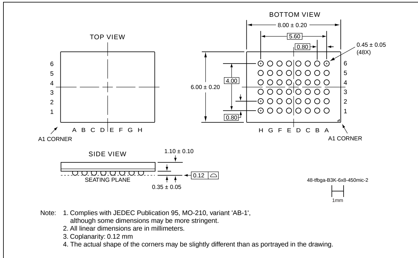
48-BALL THIN-PROFILE, FINE-PITCH BALL GRID ARRAY (TFBGA) 6MM X 8MM SST PACKAGE CODE: B3K
