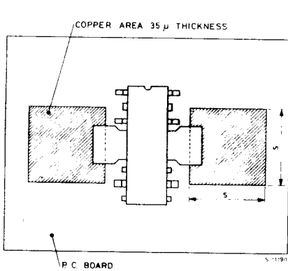
Fig. 17 - TBA 810CB mounting example
