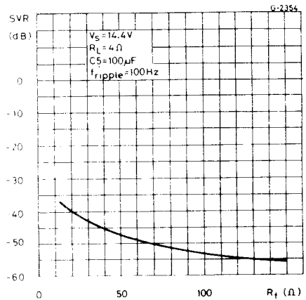
Fig. 12 - Supply voltage rejection ratio vs. feedback resistance
