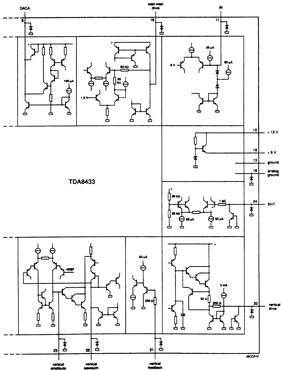
Fig.11 Input/output pin-configuration of TDA8433 (continued from Fig.10).
