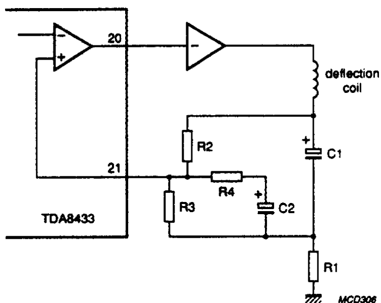
Fig.8 Application diagram of an AC coupled amplifier stage.
