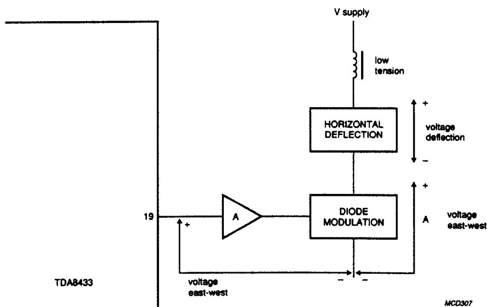
Fig.9 Application diagram for driving the diode modulator.
