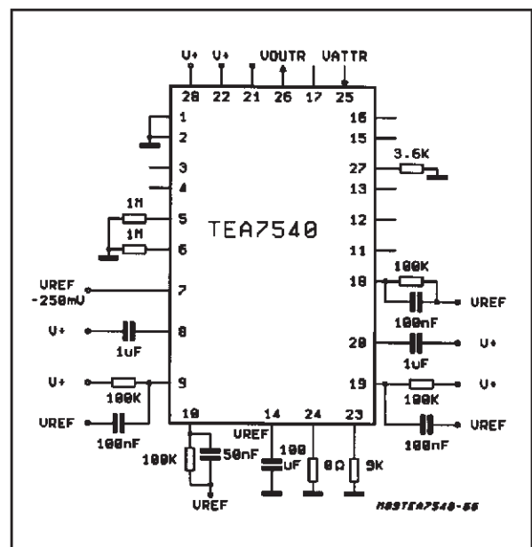
Figure 14: Test Configuration
