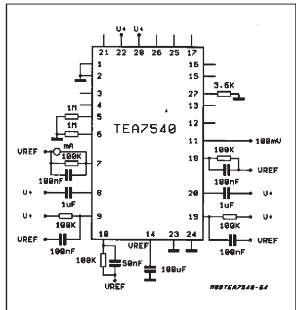
Figure 12: Test Configuration
