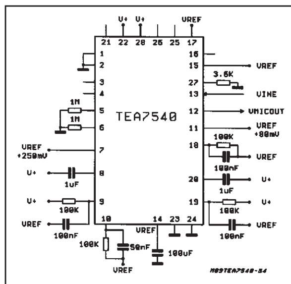
Figure 2: Test Configuration
