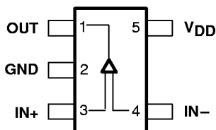
TLV2771 DBV PACKAGE (TOP VIEW)
