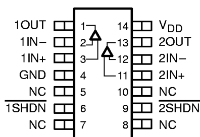
TLV2773 D OR N PACKAGE (TOP VIEW)
