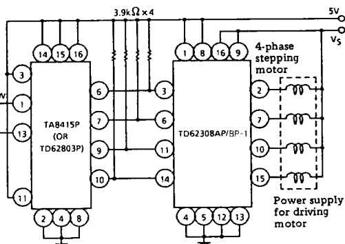
(3) Micro step driver for PPC and printer (TA8435H), PWM chopper type
