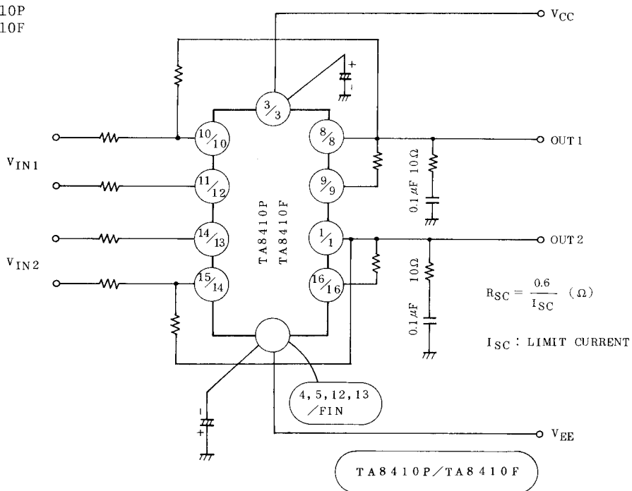
APPLICATION CIRCUIT 1
