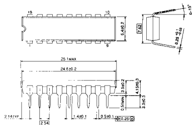
○ DIP 18-P-300D
