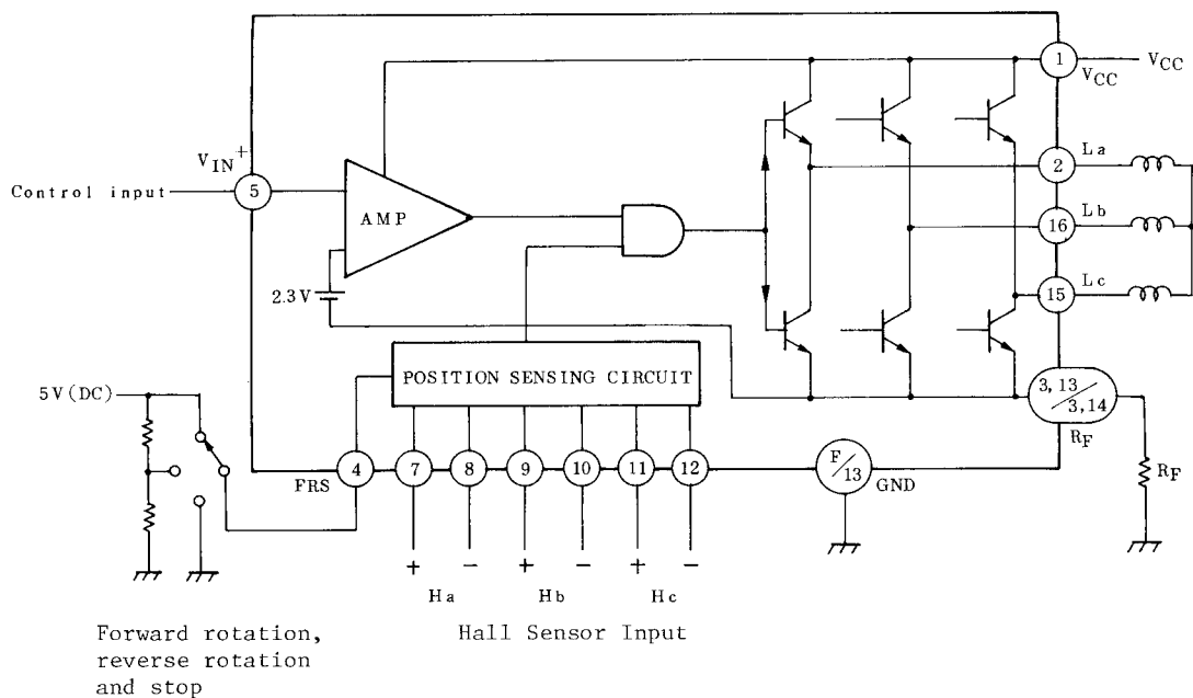
BLOCK DIAGRAM (TA8423F/TA8423P)
