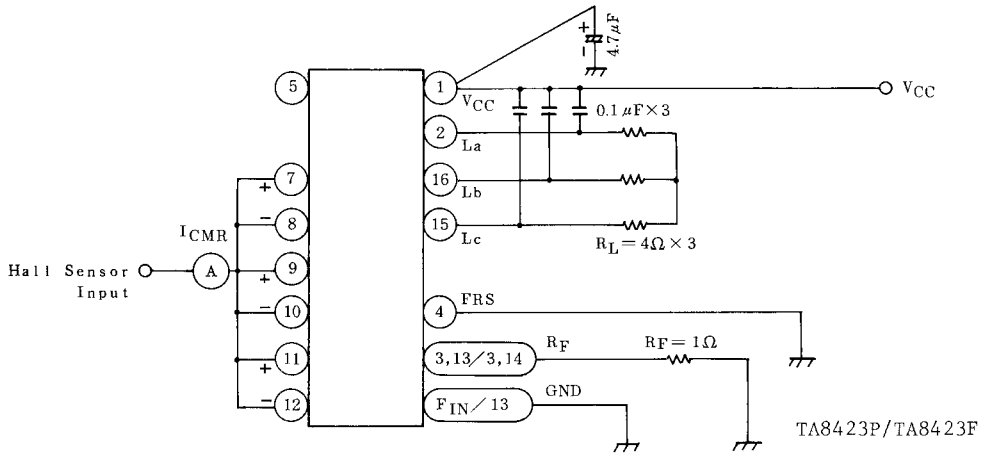
TEST CIRCUIT 3
