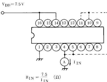
(6) Pullup resistor R_{IN}
