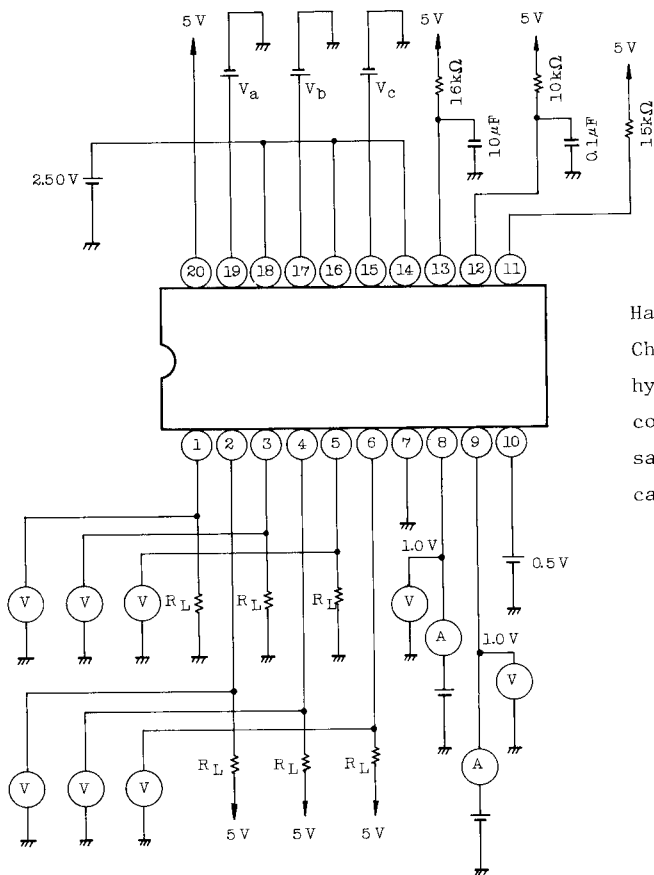
TEST CIRCUIT 2
