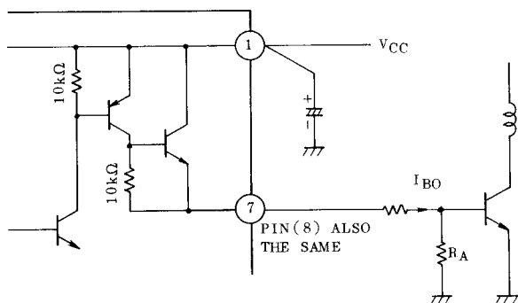
Fig. 2 Output Circuit
