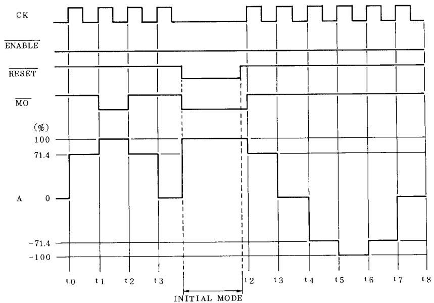
Fig. 2 1-2 Phase drive mode (M1:H, M2:L)
