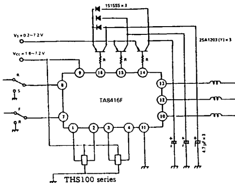
5) Portable VCR head motor drive circuit (TA8416F)
