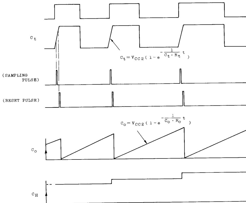
Fig. 11 TIMING CHART
