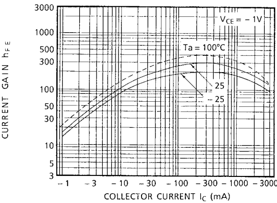
TRANSISTOR (RN6006) h_{FE} - I_C (UPPER SIDE)
