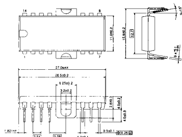
○ HDIP 14-P-500A
