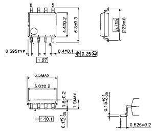
○ SOP 8-P-225
