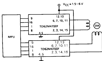
(4) Low-voltage high-efficiency stepping motor drive circuit (TD62M4700F x 2)
