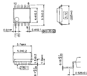
○ SSOP 10-P-225
