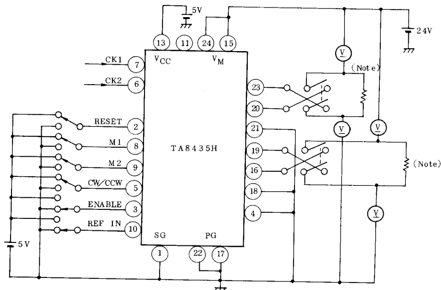
TEST CIRCUIT-4: V_{SAT-U}, V_{SAT-L}
