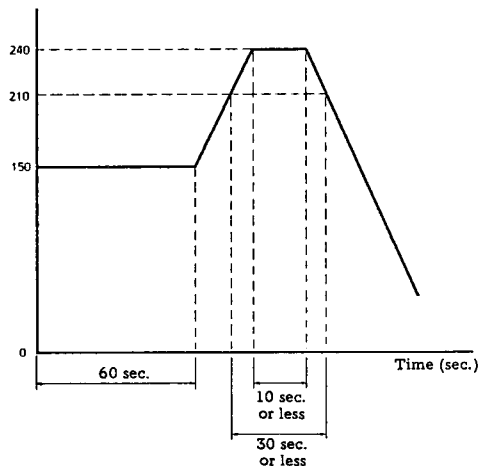
Fig. 5-6 Recommended temperature profile for reflow soldering
