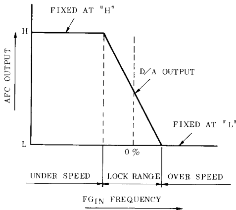
CHANGE OF APC OUTPUT AGAINST FG IN FREQUENCY
