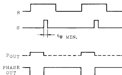
TEST WAVE
