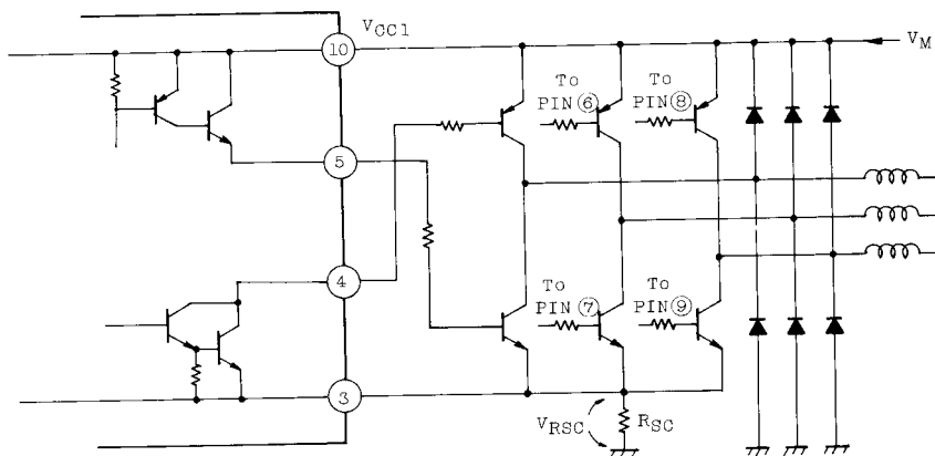
Fig. 7 OUTPUT CIRCUIT
