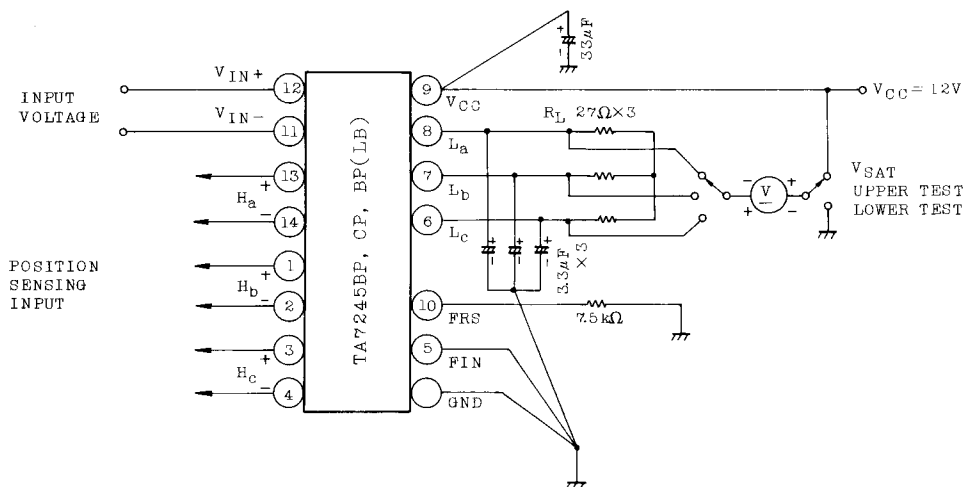
TEST CIRCUIT 2
