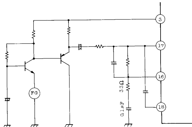
Fig. 3 FRONT AMPLIFIER
