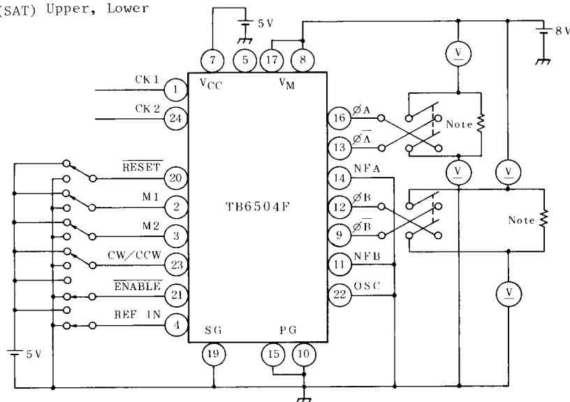
TEST CIRCUIT 4
