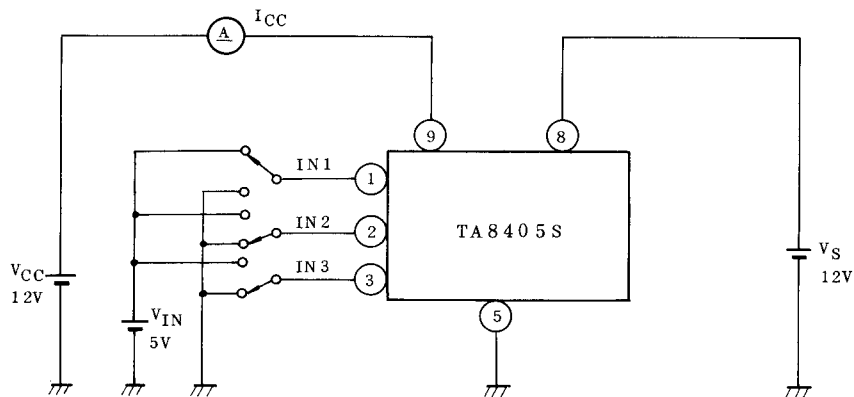
TEST CIRCUIT 1
