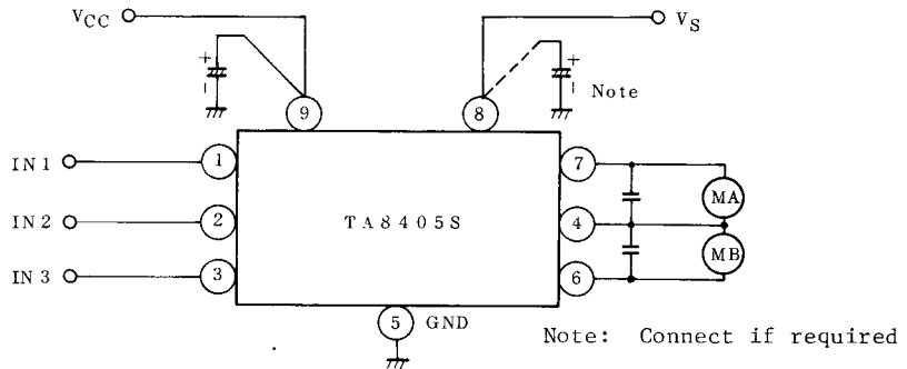
APPLICATION CIRCUIT
