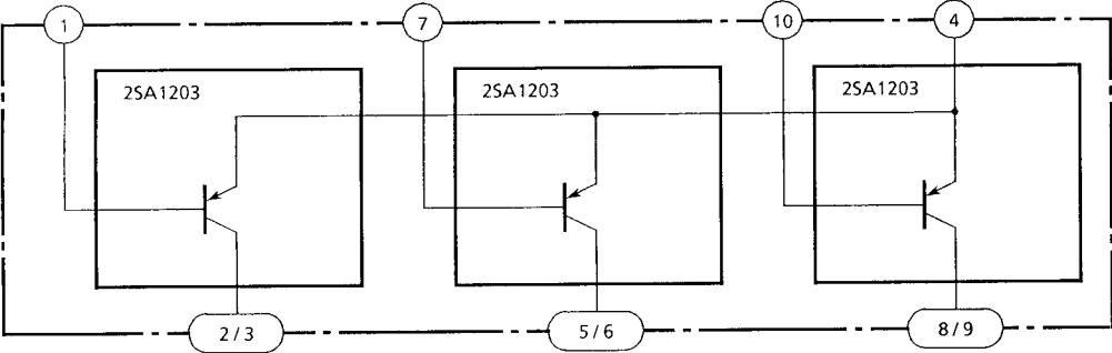
BLOCK DIAGRAM
