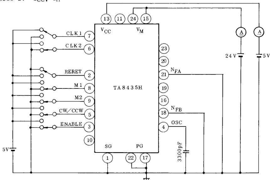
TEST CIRCUIT-2: I_{CC}, I_M
