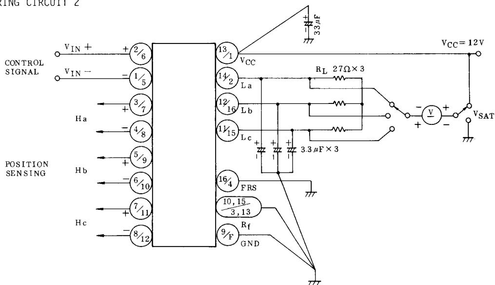
MEASURING CIRCUIT 2
