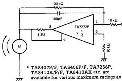
(6) Linear bridge driver (dual-power operational amplifier) (TA7272P)
