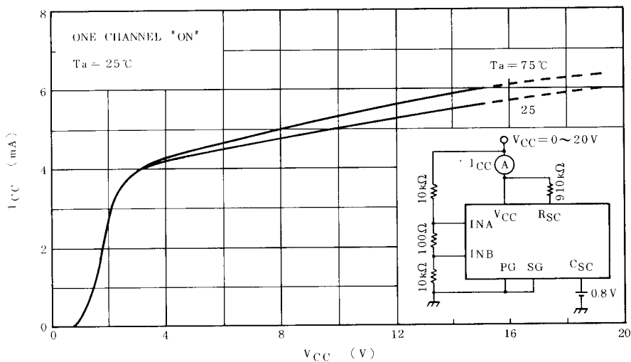
QUIESCENT CURRENT - V_{CC}
