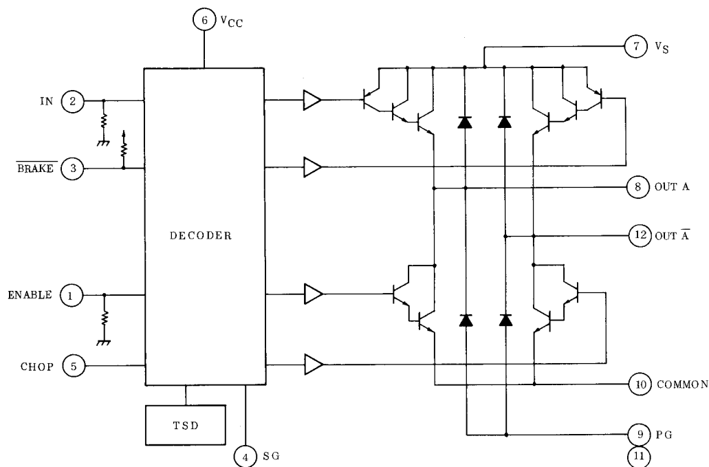
BLOCK DIAGRAM
