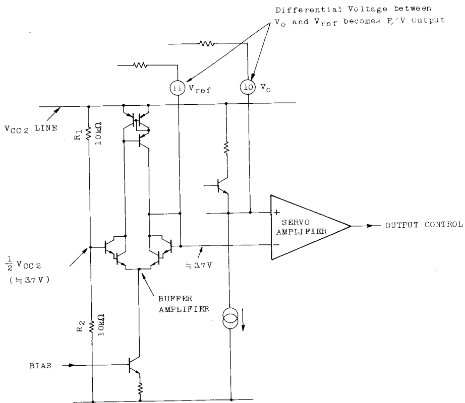
Fig. 7 VOLTAGE REFERENCE
