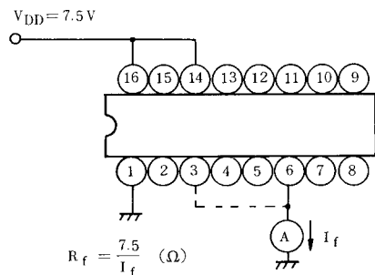
(5) Amplifier feedback resistor R_f
