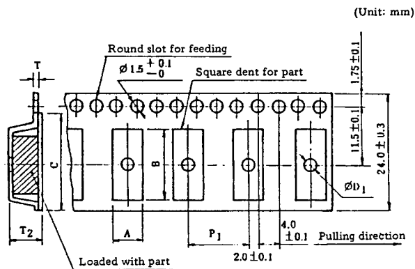
Fig. 6-7 Embossed taping types TE2412, 2416 and 2420
