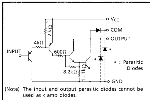
SCHEMATICS (EACH DRIVER)
