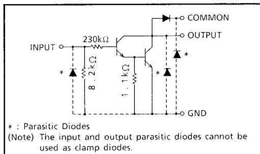
SCHEMATICS (EACH DRIVER)
