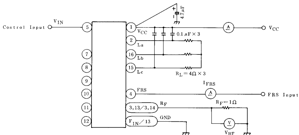
TEST CIRCUIT 1
