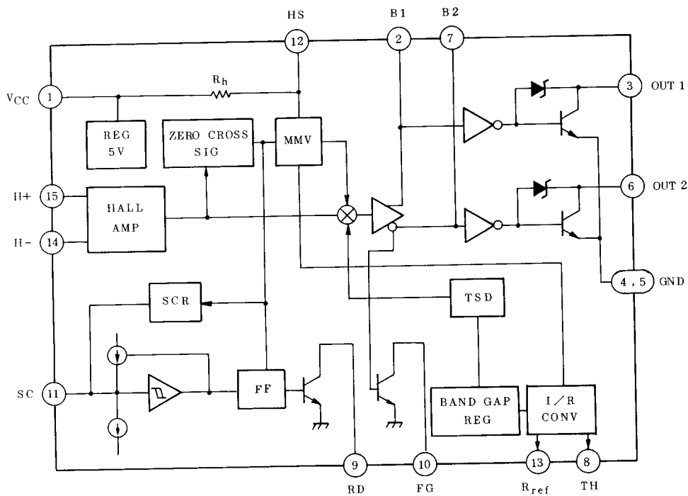
BLOCK DIAGRAM
