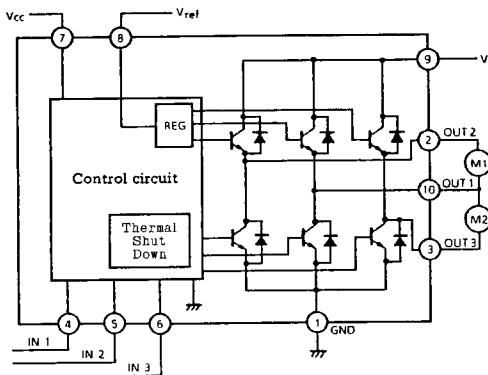
(4) Large current single-bridge driver (TA8429H)
