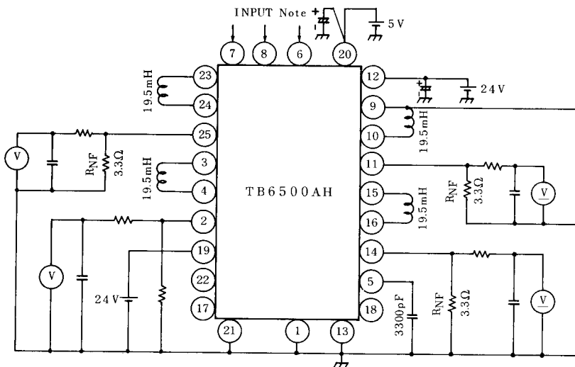
TEST CIRCUIT 6. V_{\text{refH}} , V_{\text{refL}} , \Delta V_{\text{ref}}
