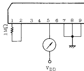
TEST CIRCUIT (1)
