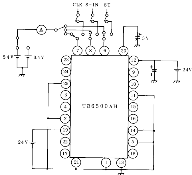
TEST CIRCUIT 6. V_{\text{refH}} , V_{\text{refL}} , \Delta V_{\text{ref}}
