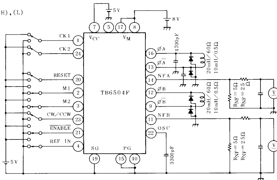
TEST CIRCUIT 4
