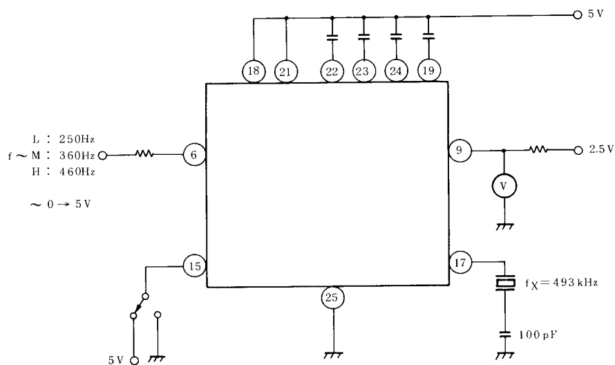
TEST CIRCUIT 6 V_{PWM-H} , V_{PWM-M} , V_{PWM-L}
