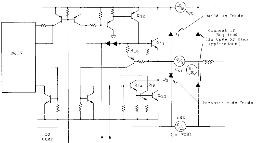
Fig. 4 OUTPUT CIRCUIT
