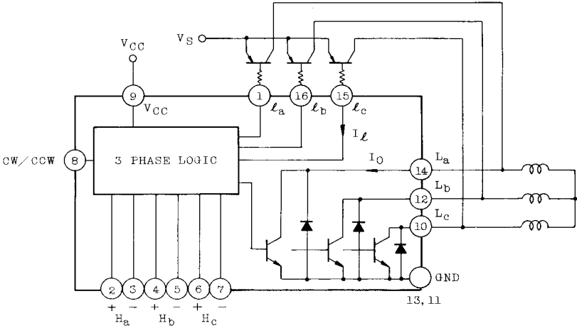
BLOCK DIAGRAM
