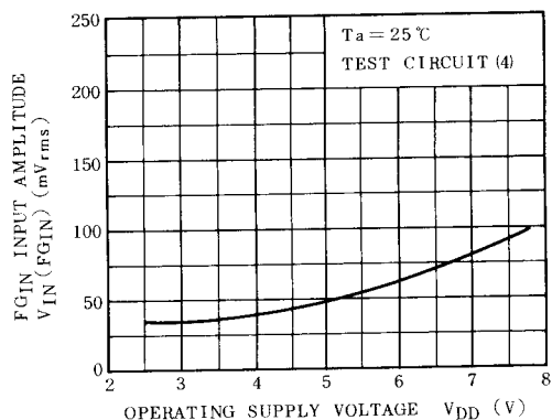
V_{\text{IN}}(\text{FG}_{\text{IN}}) - V_{\text{DD}}
