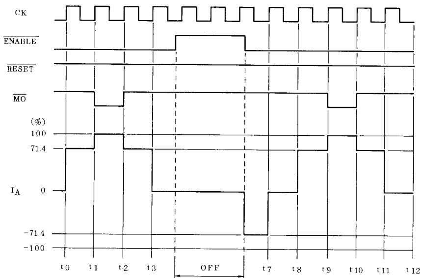
Fig.1 1-2 Phase drive mode (M1:H, M2:L)
