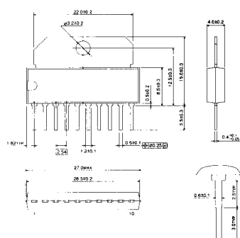
○ HSIP 10-P
