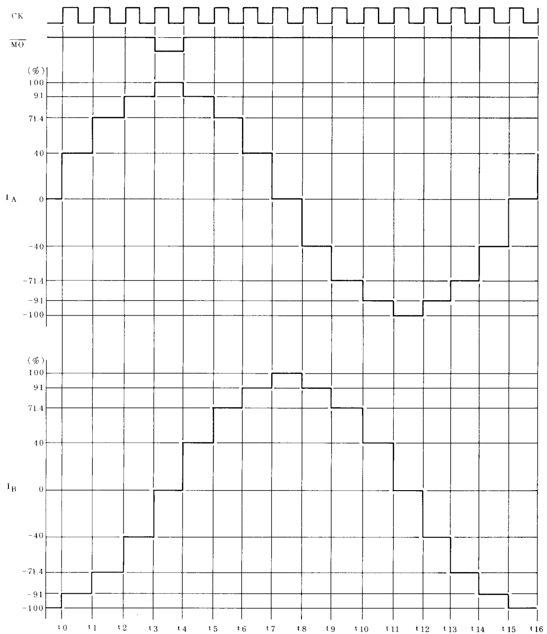
W1-2 Phase Excitation (M1:L, M2:H, CW Mode)
