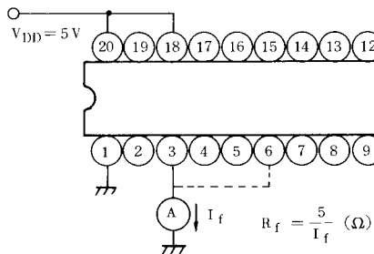
(5) Amplifier Feedback Resistance ( R_f )
