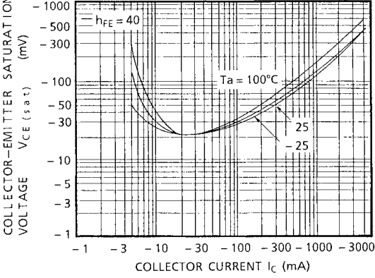
TRANSISTOR (RN6006) V_{CE(sat)} - I_C
