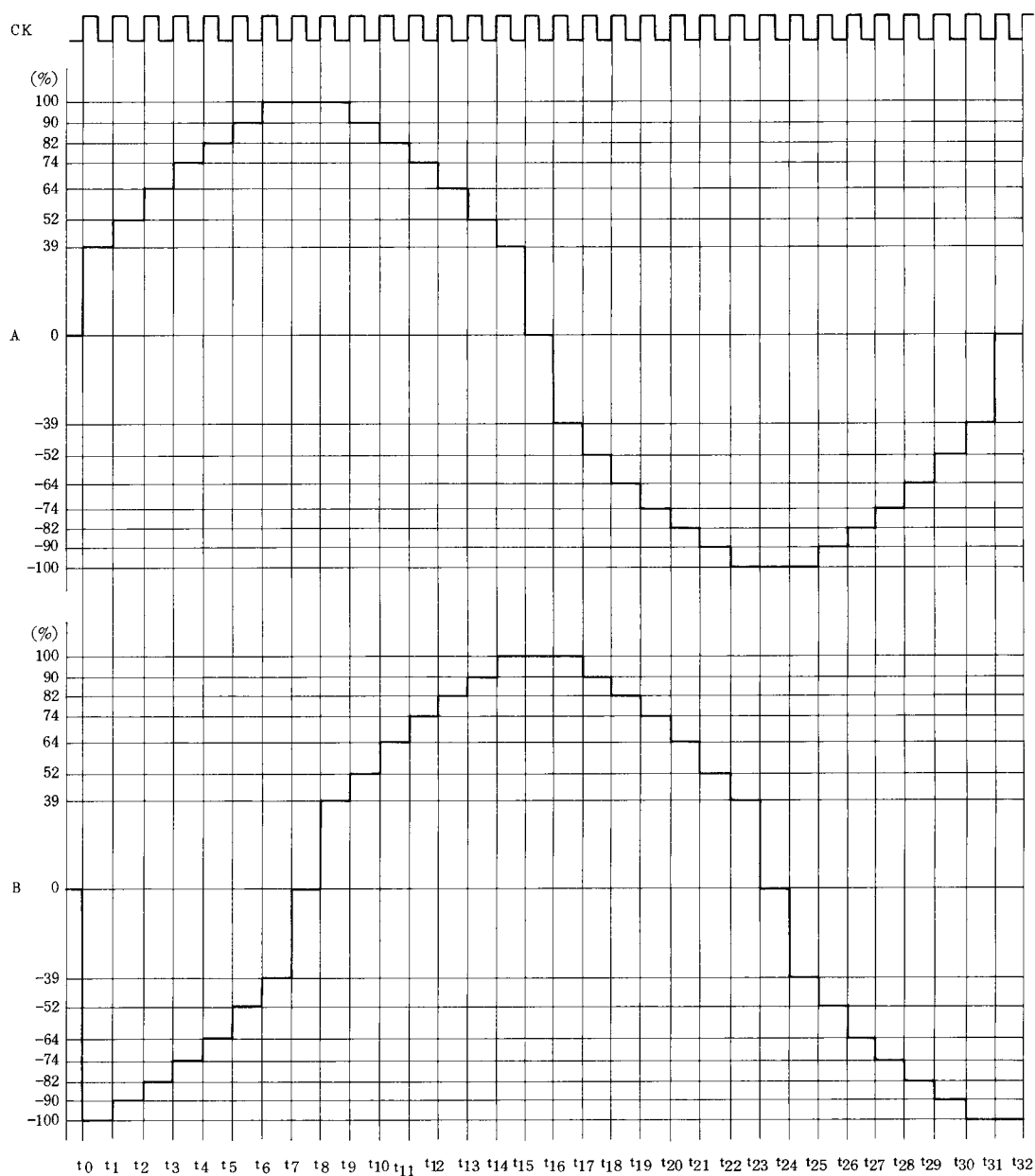
2W1-2 Phase Excitation (M1:H, M2:H)
