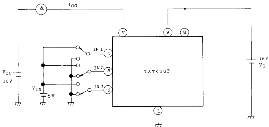
TEST CIRCUIT 1
