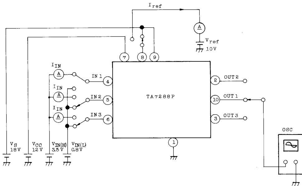
TEST CIRCUIT 2
