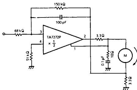
(6) Linear bridge driver (dual-power operational amplifier) (TA7272P)
