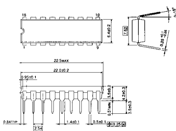
○ DIP 18-P-300A
