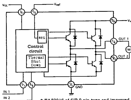
(1) Output voltage adjusting-type single-bridge driver (TA7291P/F)
