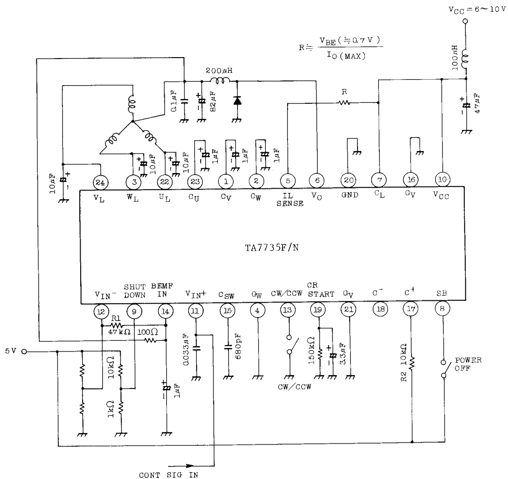
APPLICATION CIRCUIT 2.
