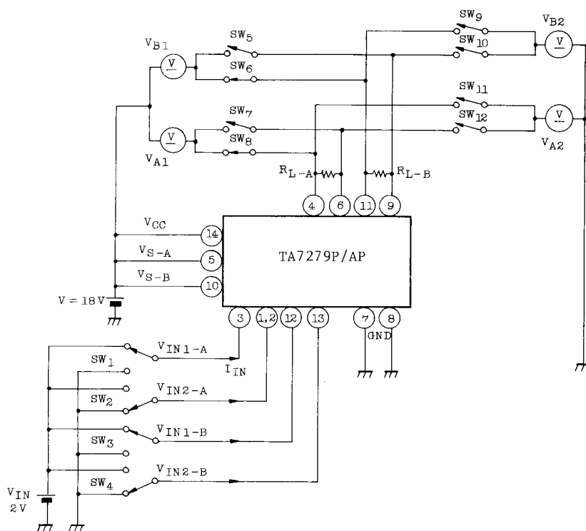
MEASURING CIRCUIT 4. V_{F-U,L}
