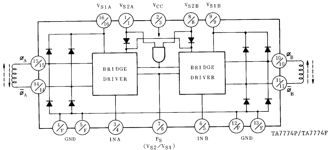
BLOCK DIAGRAM
