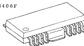
HSOP16-P-300
