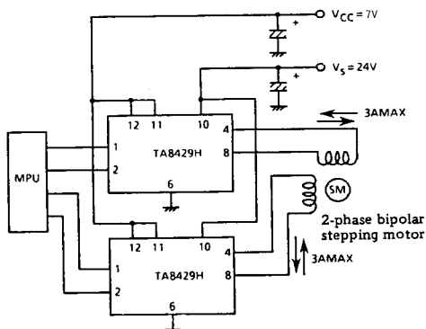
(5) Large-current stepping motor drive circuit (TA8429H x 2)
