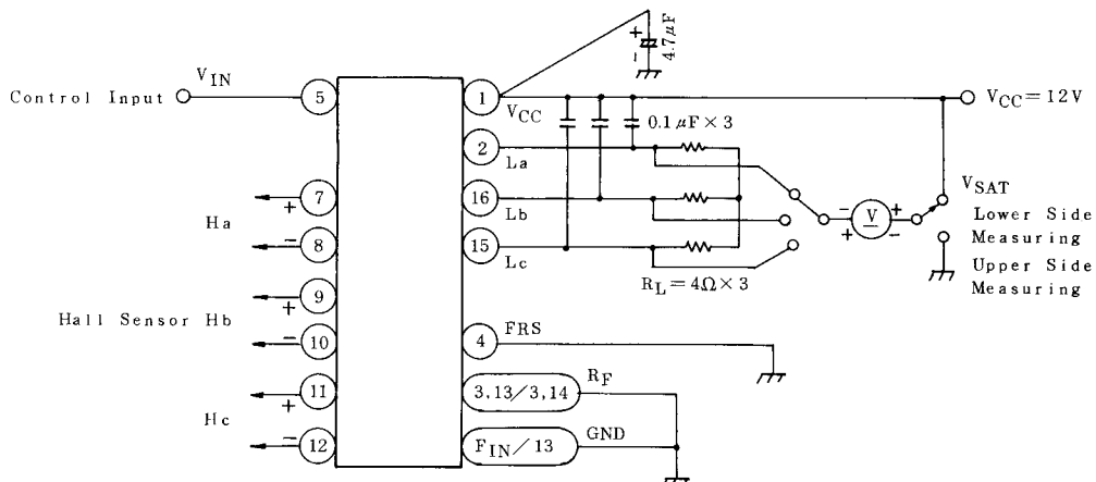
TEST CIRCUIT 2
