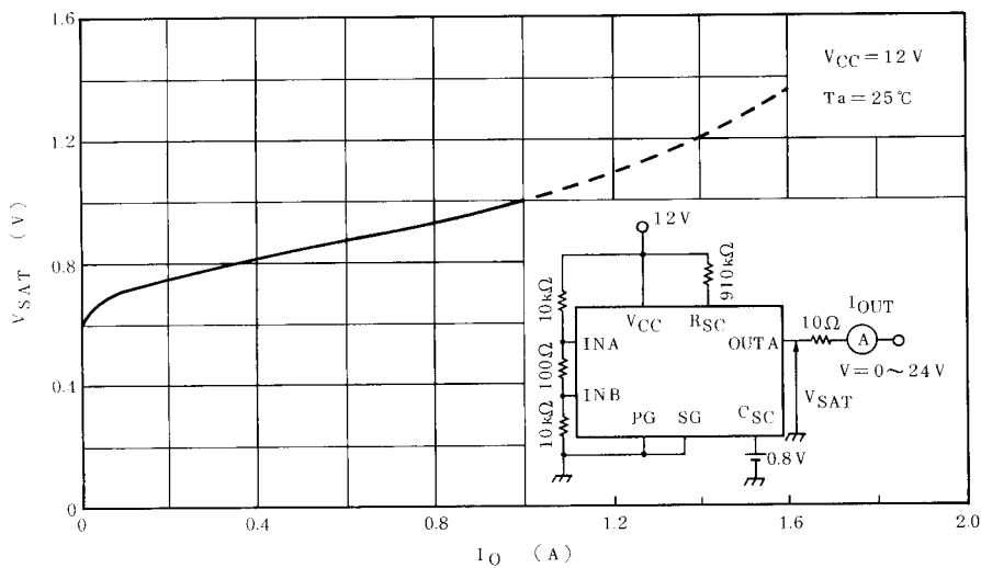
OUTPUT SATURATION - I_O
