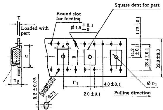
Fig. 6-8 Embossed taping types TE3212, 3216, 3220, 3224, 3228, and 3232
