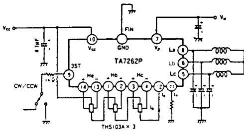
1) Voltage-control type capstan (head) motor drive circuit (TA7262P/F)
