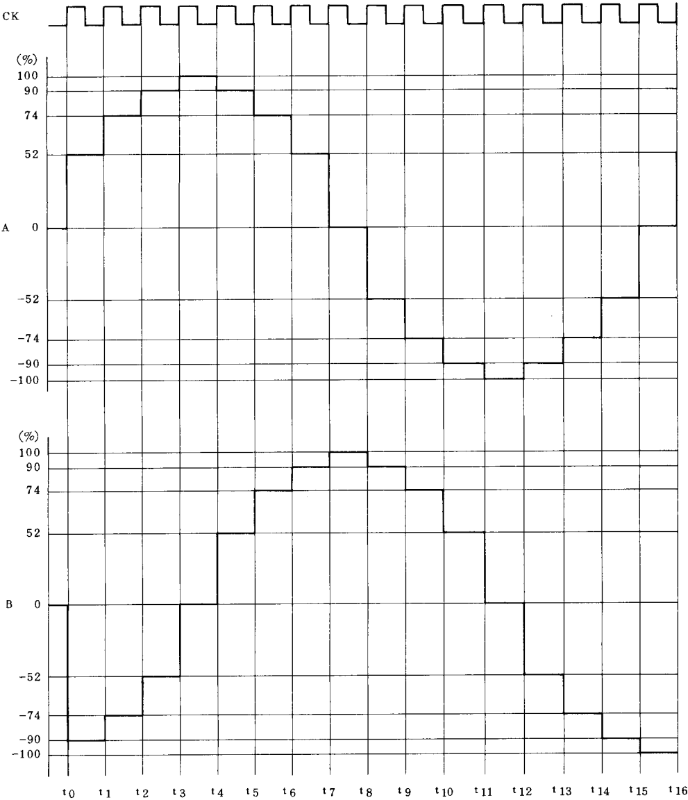
W1-2 Phase Excitation (M1:L, M2:H)
