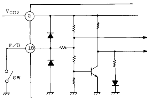
Fig. 6 FORWARD/REVERSE ROTATION SELECTOR CIRCUIT
