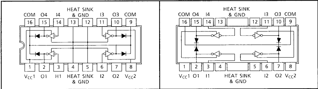
SCHEMATICS (EACH DRIVER)
