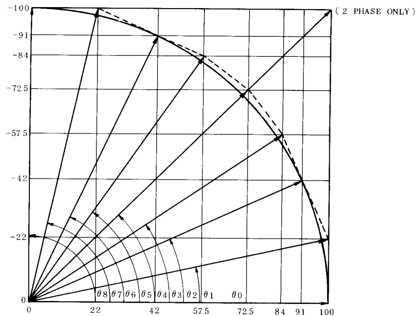
OUTPUT CURRENT VECTOR ORBIT (NORMALIZE TO 90 DEG FOR EACH ONE STEP)
