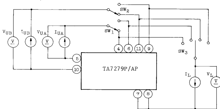
MEASURING CIRCUIT 4. V_{F-U,L}
