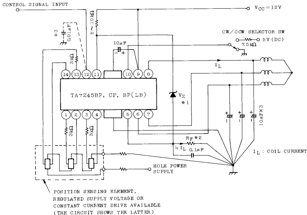
TA7245BP APPLICATION CIRCUIT 1
