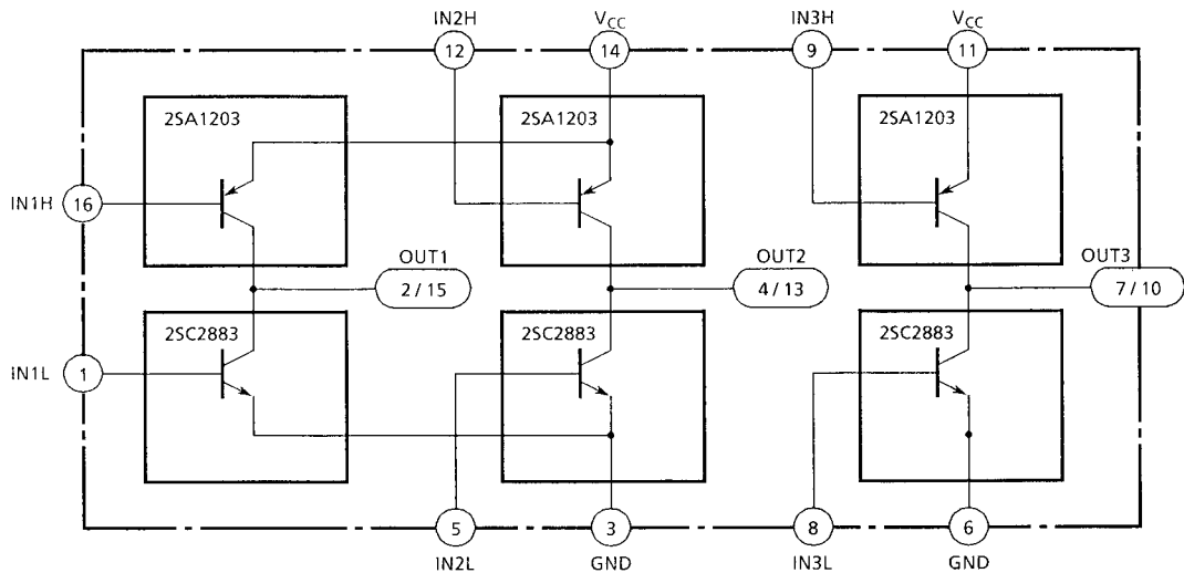
INTERNAL BLOCK CONNECTION
