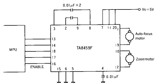
6) Auto-focus/zoom motor driver circuit for movie cameras (Smart MOS TA8459F)
