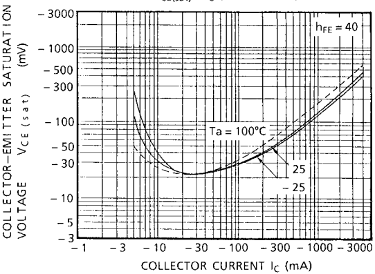
TRANSISTOR (RN6006) V_{CE(sat)} - I_C (LOWER SIDE)
