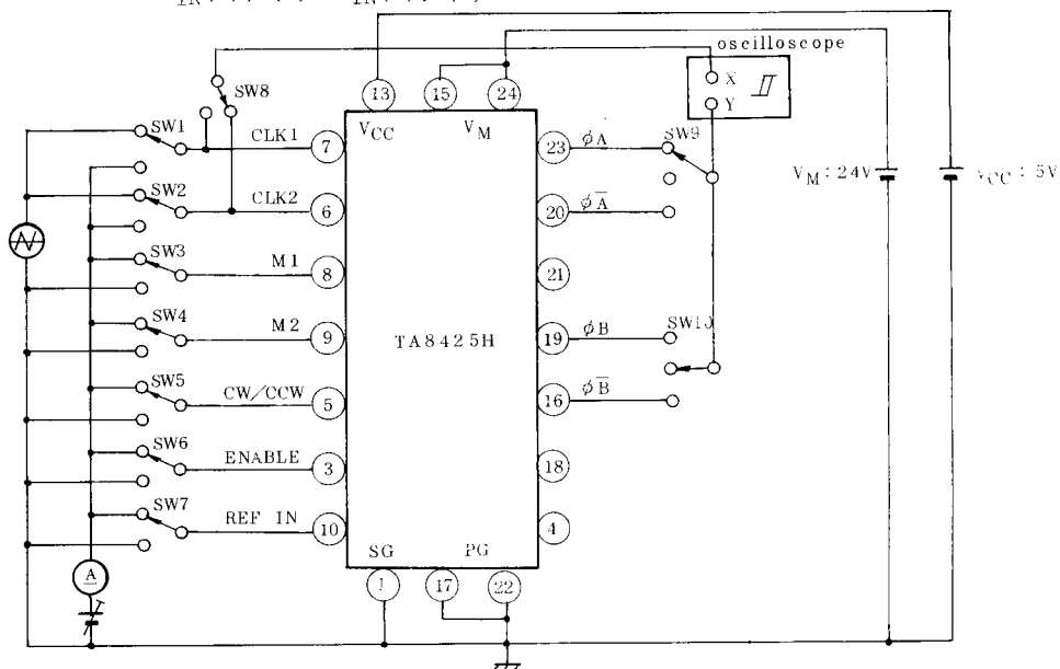
TEST CIRCUIT-1: V_{IN(H)}, (L) \cdot I_{IN(H)}, (L)
