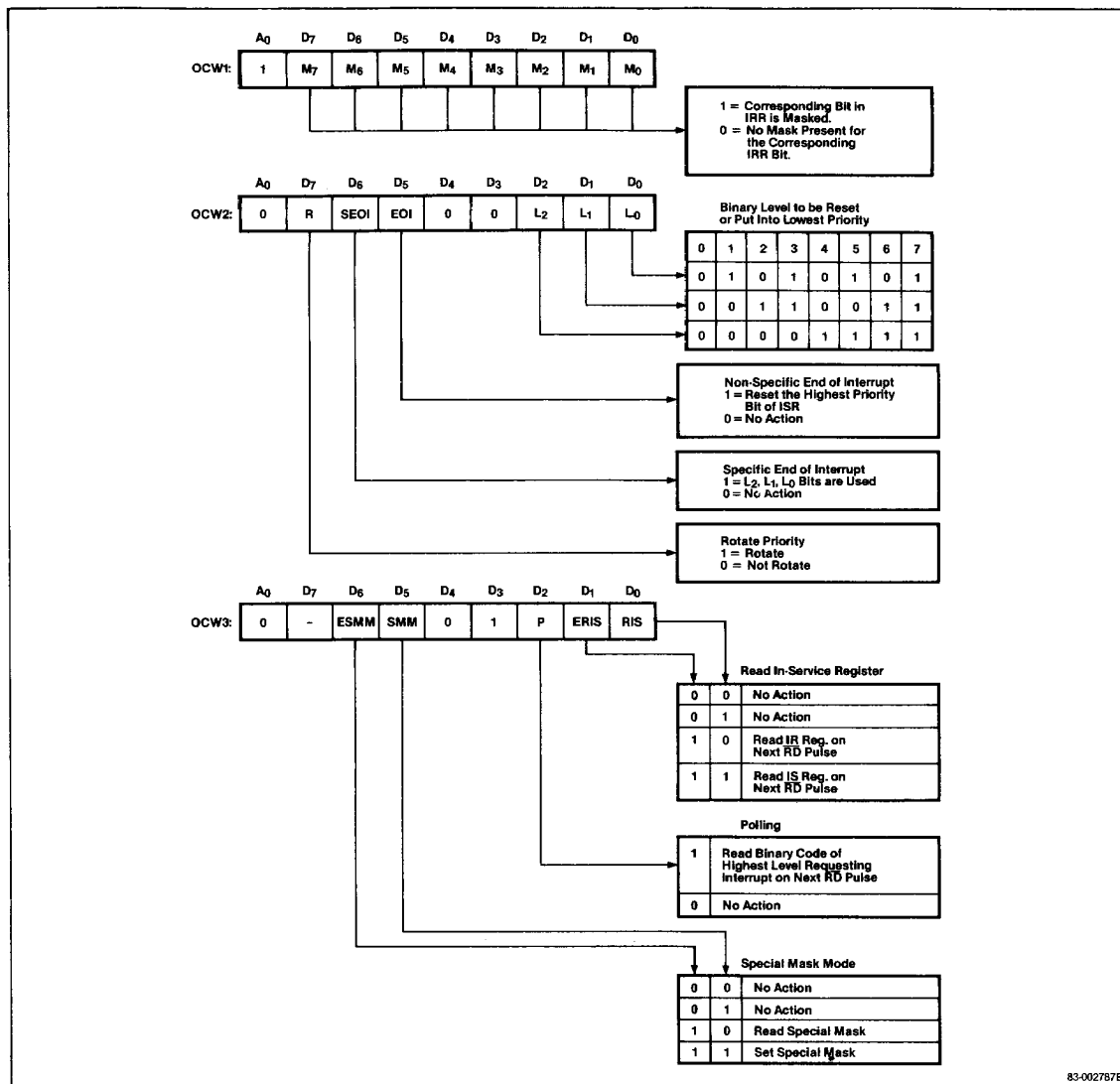
Figure 3. Operation Command Word Format
