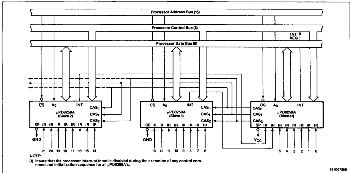
Figure 4. Cascading the μPD8259A
