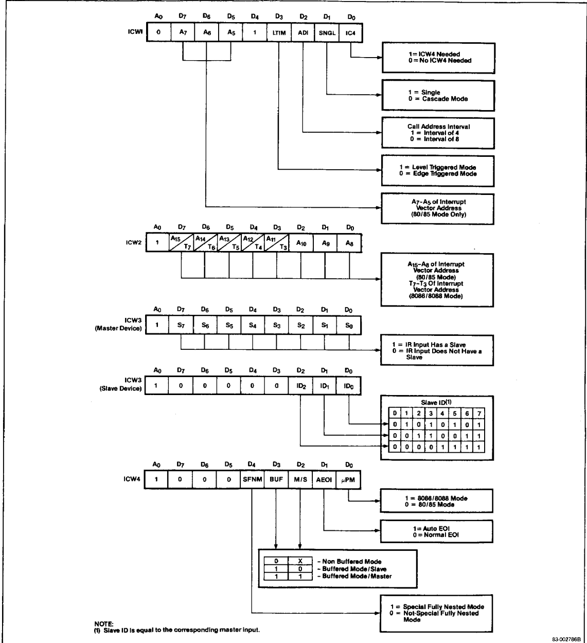
Figure 2. Initialization Command Word Format
