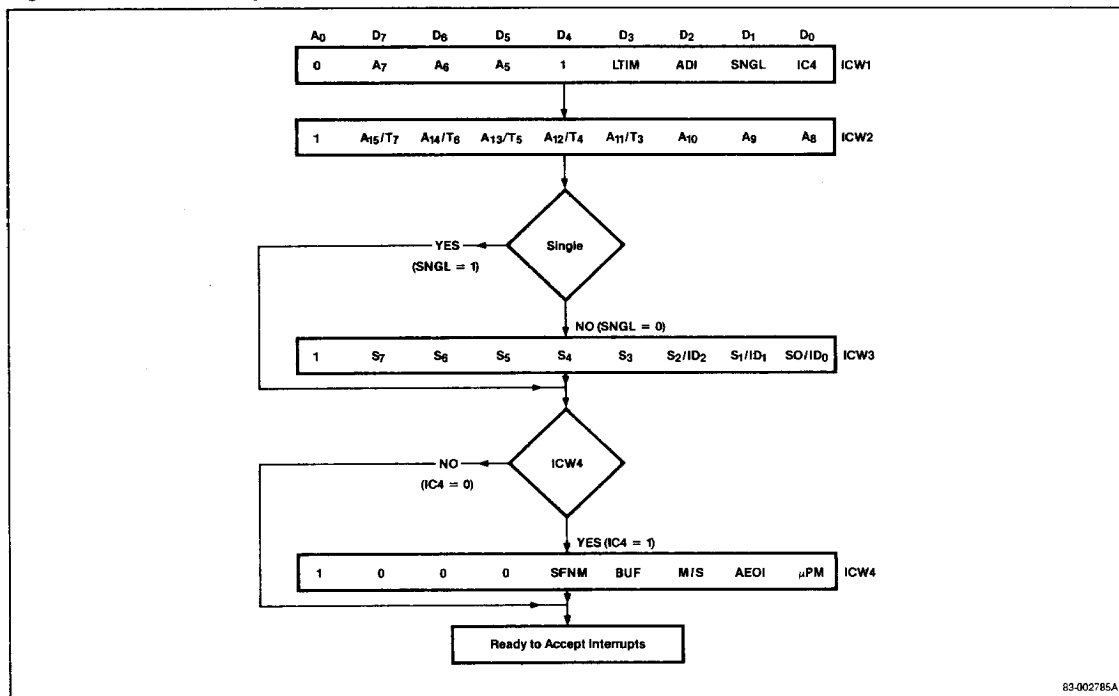
Figure 1. Initialization Sequence
