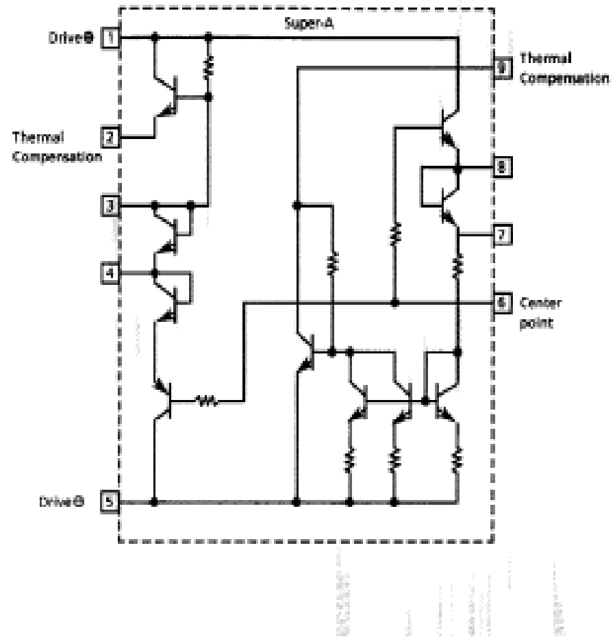
(2) Block Diagram
