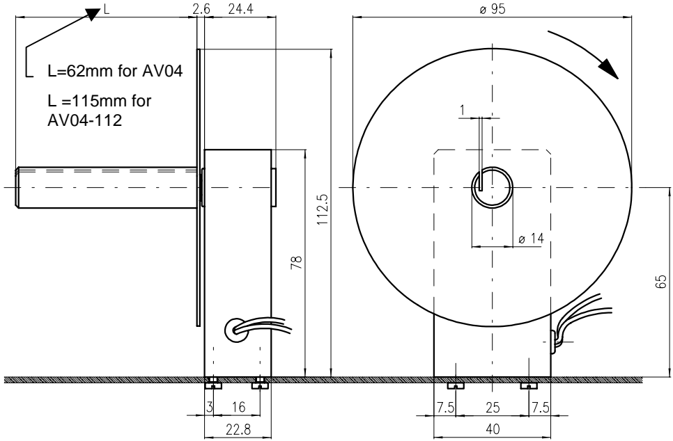
AV04/AV04-112 OVERALL DIMENSIONS
