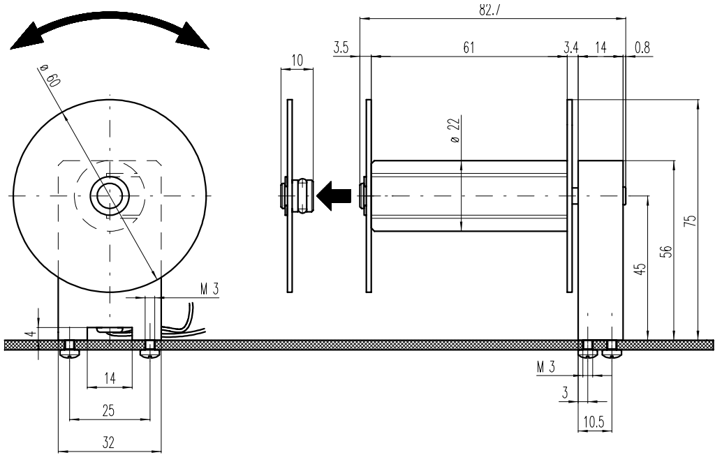
AV03-0023 OVERALL DIMENSIONS
