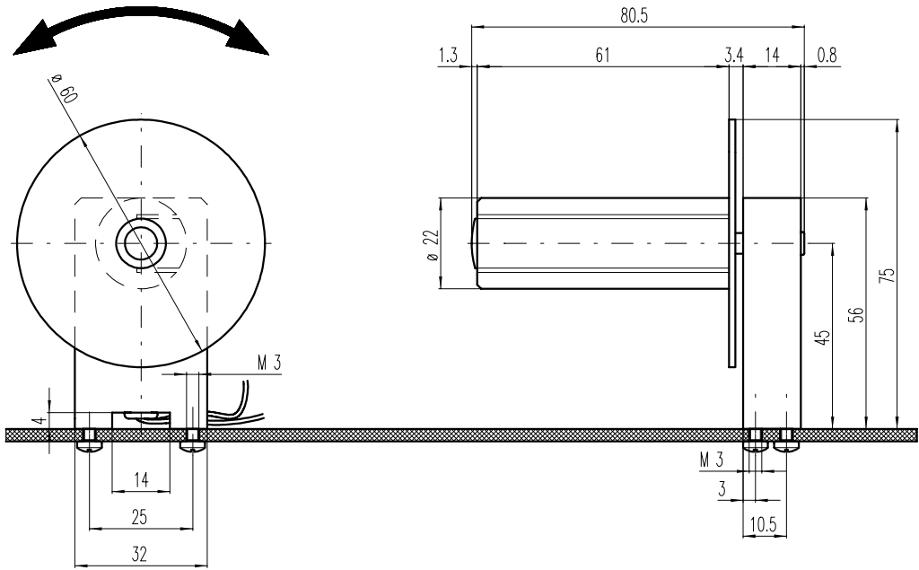
AV03-0060 OVERALL DIMENSIONS
