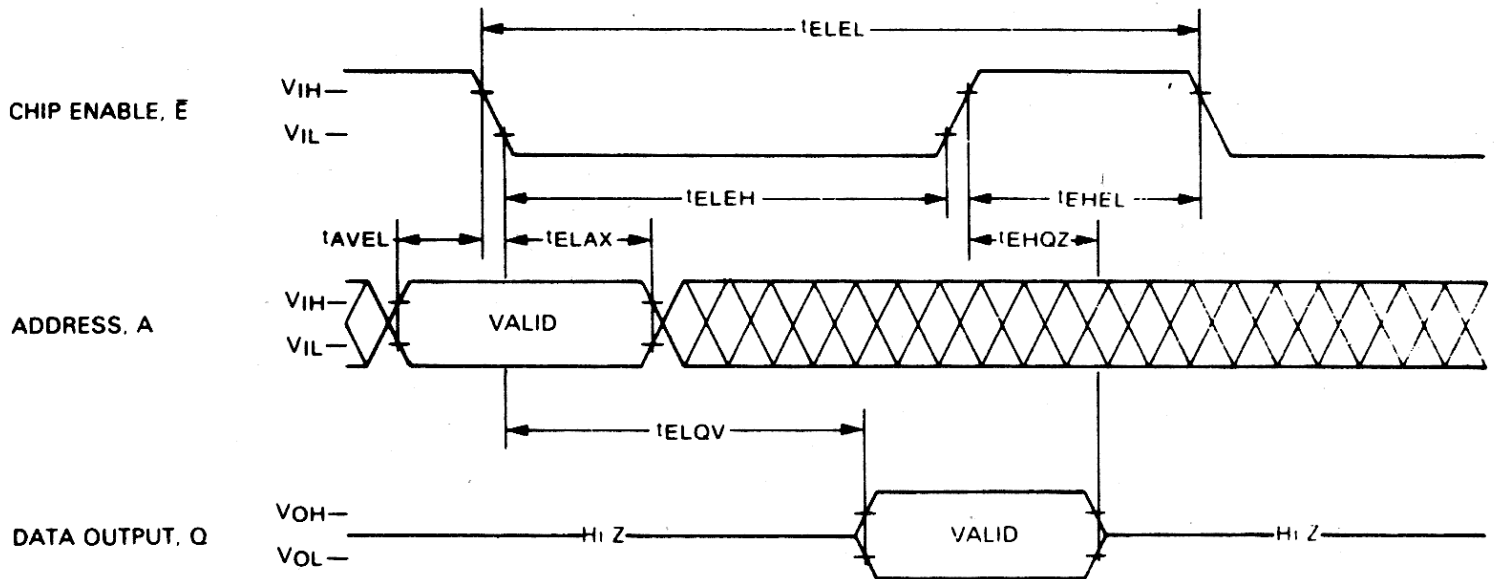
FIGURE 2 – TIMING DIAGRAM
