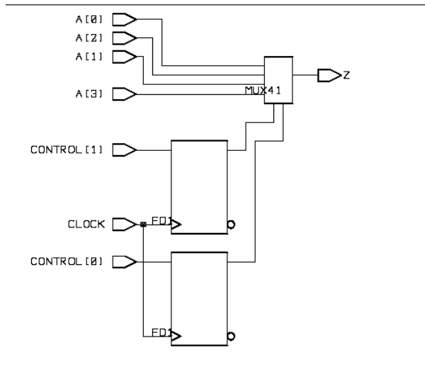
Figure 8-16 Two Processes: One Synchronous, One Asynchronous
