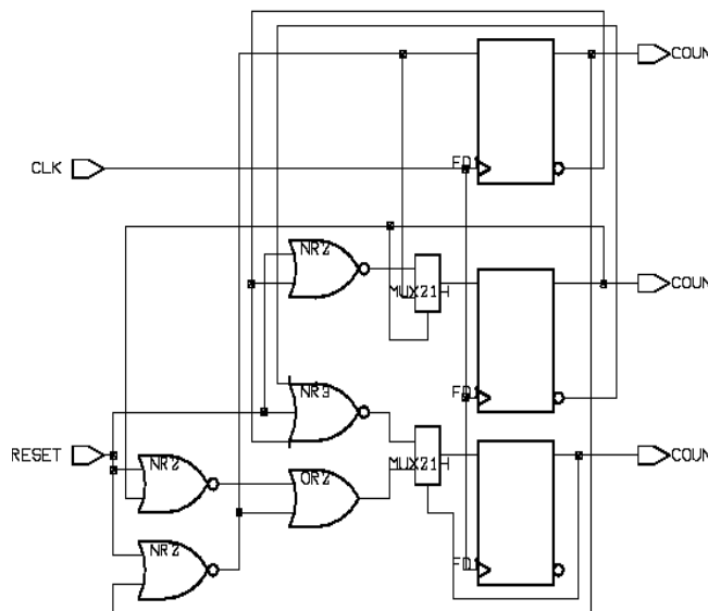
Three-Bit Counter Schematic
