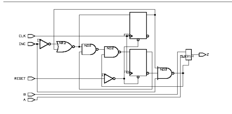
Synchronous Finite State Machine with Asynchronous Reset
